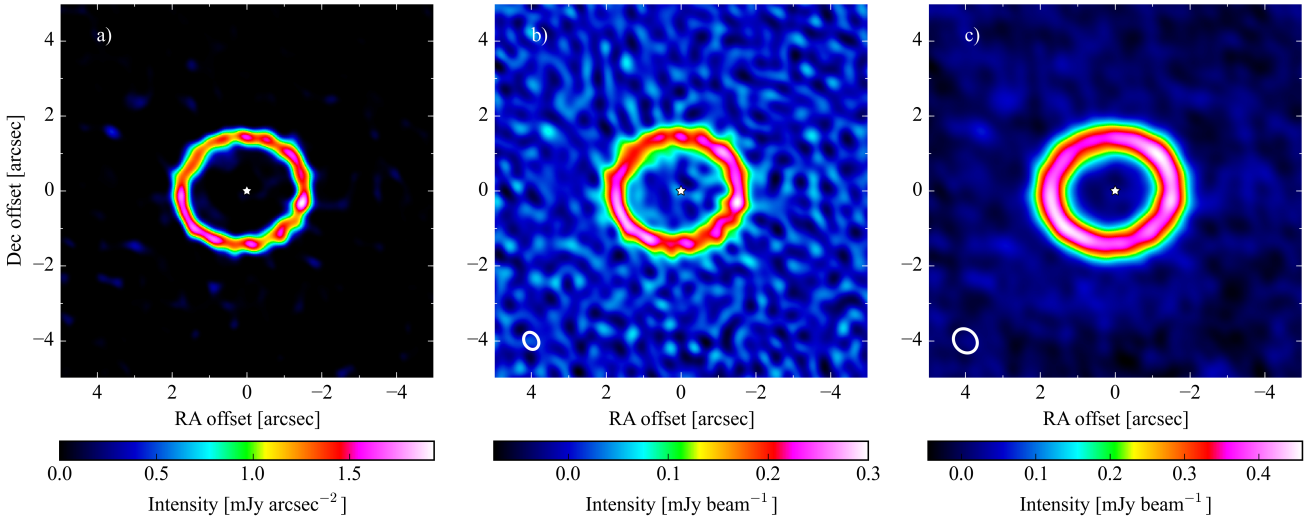
Figure 1. ALMA dust continuum maps at 220 GHz (Band 6). a) panel: MEM non-parametric model (regularized with the maximum entropy method). b) panel: restored image adding residuals and convolving with a synthetic beam corresponding to Briggs weighting ( 0''.47 \times 0''.36 ). c) panel: restored image adding residuals and convolving with a synthetic beam corresponding to natural weighting ( 0''.69 \times 0''.58 ). The respective beams are represented by white ellipses. The x- and y-axes indicate the offset from the stellar position in R.A. and decl. in arcsec, i.e. north is up and east is left. The stellar position is marked with a white star.
