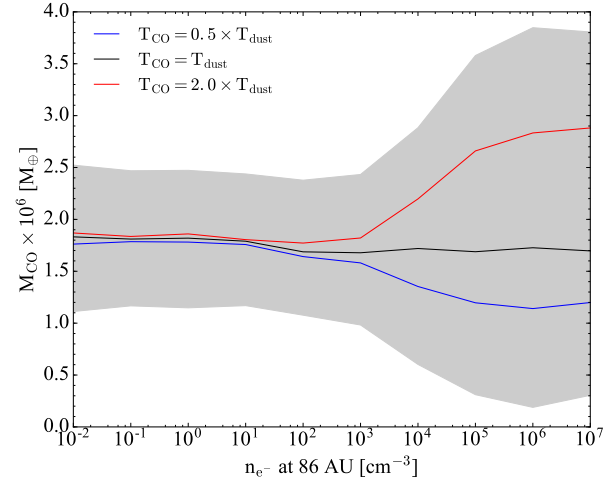
Figure 6. Best fit CO gas mass values obtained from our MCMC analysis using different kinetic temperatures and electron densities ( n_{e^-}^0 , main collisional partner). The blue, black and red lines correspond to kinetic temperatures equal to 0.5, 1 and 2.0 times the dust temperature in the disc, respectively. The grey area represents the 68% confidence region with gas temperatures ranging between 0.5 – 2.0 times the dust temperature.
