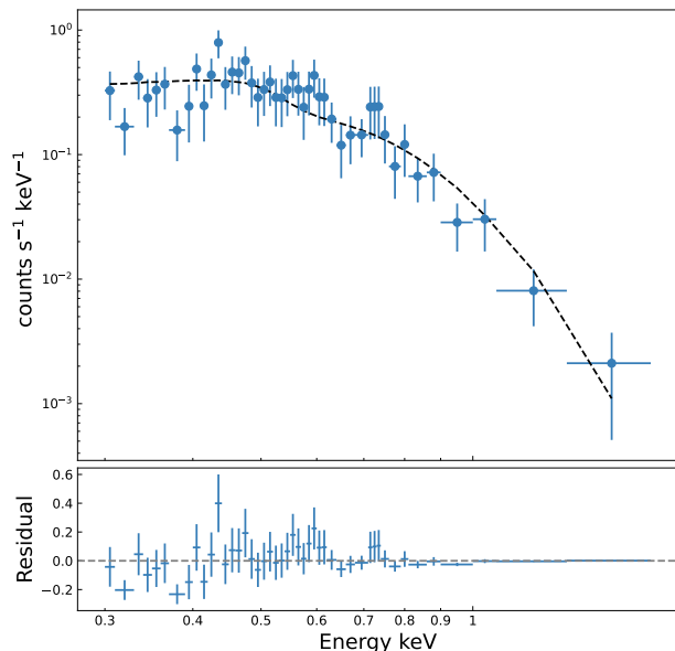
Fig. 5. Swift /XRT spectrum of the source detected at a distance of 6.0 \pm 3.6'' from the nucleus of SDSS1335+0728, obtained on February 4 2024. Top : The blue circles show the data, and the black dashed line shows the black body model with kT = 104 \pm 9 eV. Bottom : Residual of the modelling (the difference between the original spectrum and the fit).
