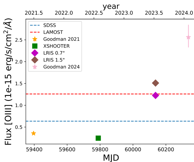
Fig. 10. Light curve of the [OIII] NEL of SDSS1335+0728 for observations obtained after December 2019. We include the measurements obtained from Goodman (yellow and pink stars), X-shooter (green square), and LRIS (magenta and brown diamonds). The horizontal dashed lines show the flux level of the SDSS and LAMOST observations.
