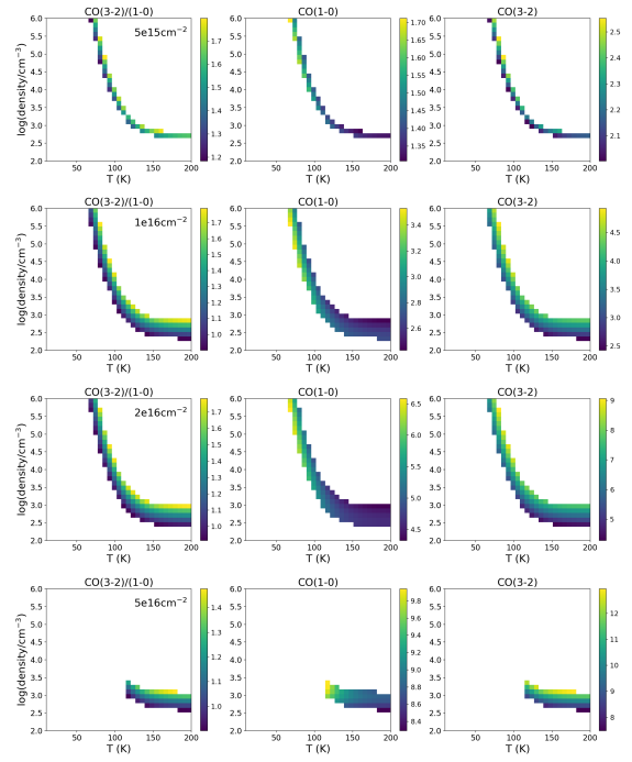
Fig. B.2. Parameter space of Radex models reproducing the 'high-excitation' line intensities and line ratios found at the western edge of the NGC 2023 and NGC 2024 cloud (see Figs. 23, 24).
