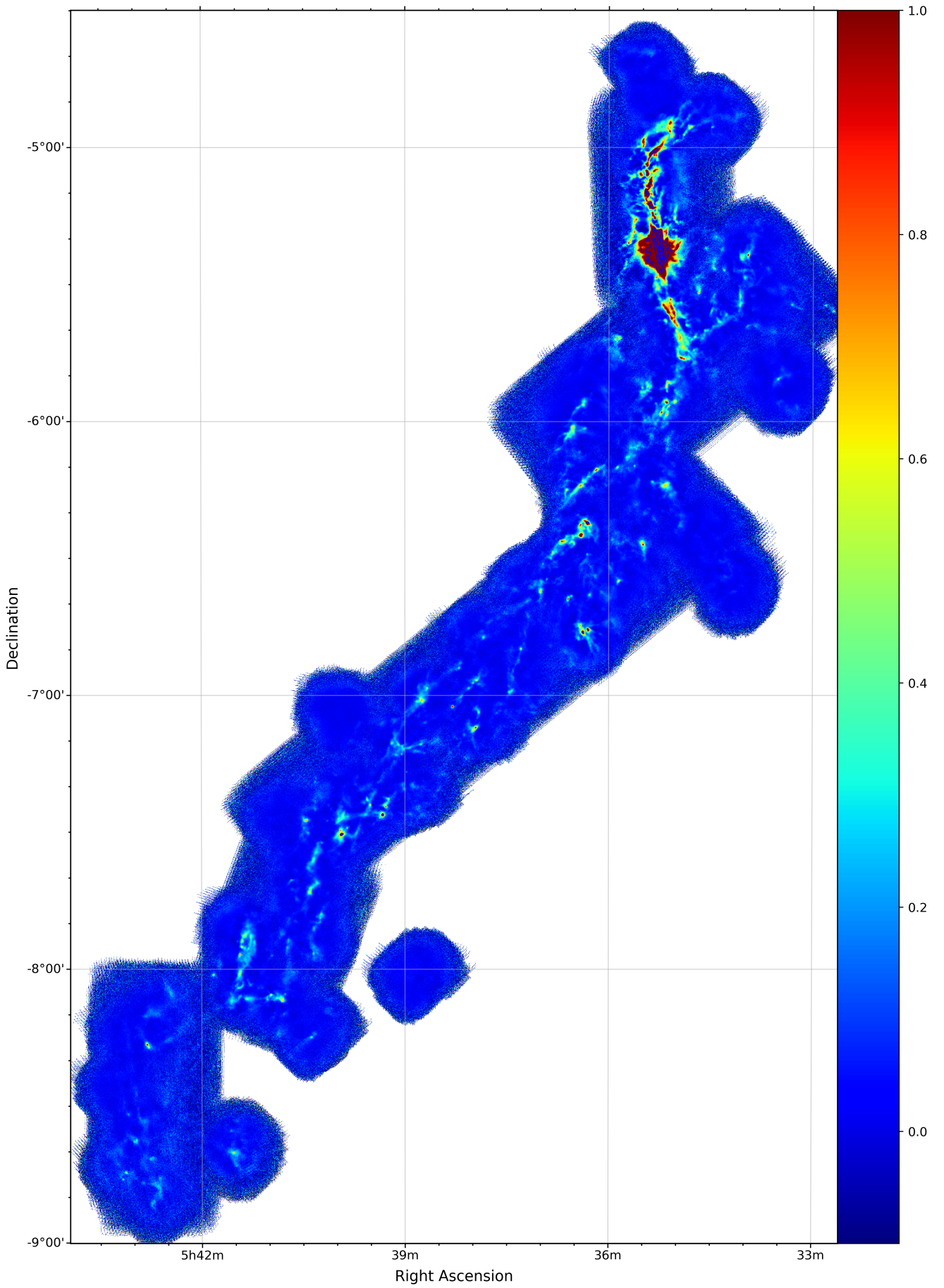
Fig. C.5. As Fig. C.1, for Orion A (including the L 1641-S CO survey field in the south).
