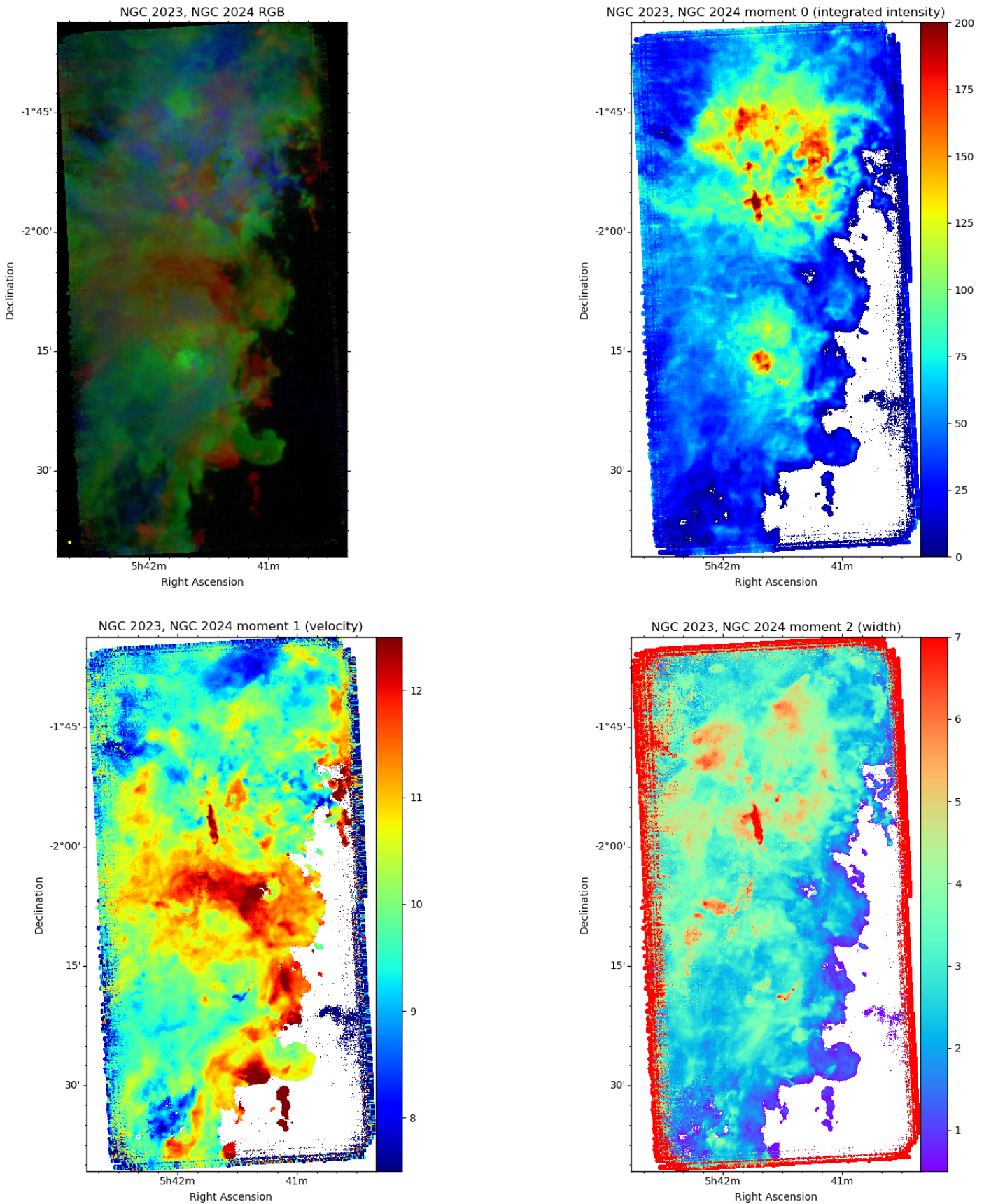
Fig. A.12. Properties of the velocity field in the NGC 2023 and NGC 2024 area. Top, left panel: red/green/blue representation of the velocity field around the clouds ambient velocity; red: v = +11.5 km/s to +14.0 km/s; green: v = +9.25 km/s to +11.25 km/s; blue: v = +6.5 km/s to +9.0 km/s. The yellow dot in the lower left corner indicates the beam size. The remaining three panels show maps of the first three moments of the line emission, computed over the velocity range from -5 km/s to +20 km/s, and limited to emission brighter than 3.5 K.
