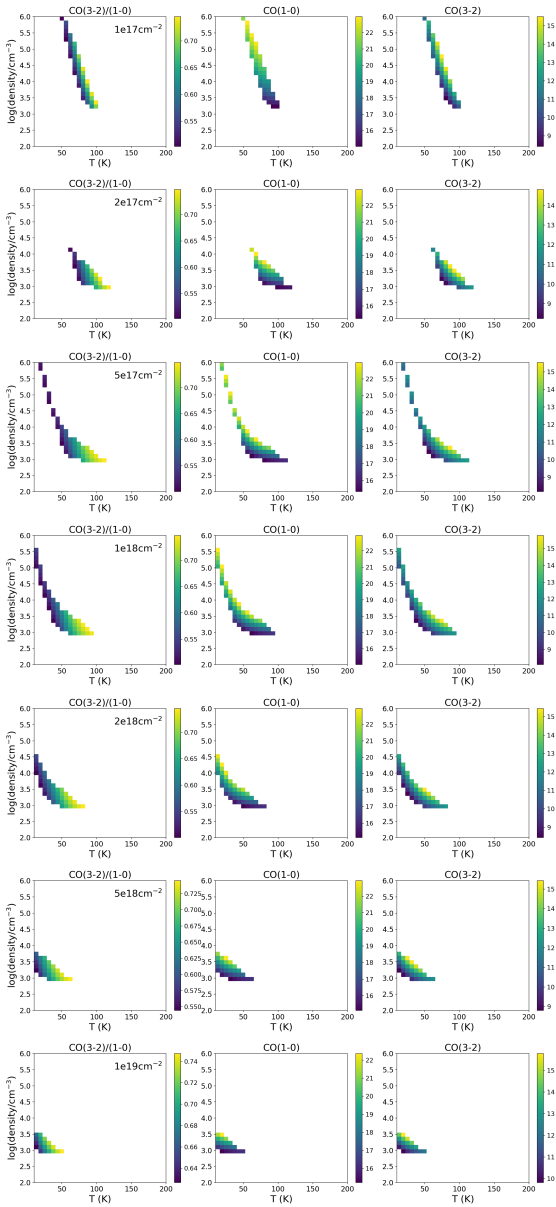
Fig. B.1. Parameter space of Radex models reproducing the 'typical' line intensities and line ratios found in the NGC 2023 and NGC 2024 region (see Figs. 23, 24).
