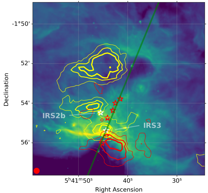
Fig. 26. Spitzer IRAC4 ( 8.0 \mu\text{m} ) image of the central NGC 2024 region (logarithmic colour scale) overlaid with contours of CO(3-2) emission at 10.75 to 11.25 km/s (yellow) and 12.75 to 13.25 km/s (red); red stars mark the positions of FIR1 to 6 from Mezger et al. (1988), the green line marks the location of the position-velocity cut shown in Fig. 25. The red circle in the lower left marks the beam size of the CO(3-2) maps.
