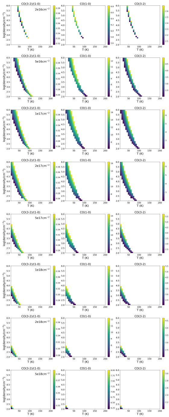
Fig. B.3. Parameter space of Radex models reproducing the line intensities and line ratios found in the velocity component around 4-5 km/s in the NGC 2023 and NGC 2024 region (see Fig. 21).
