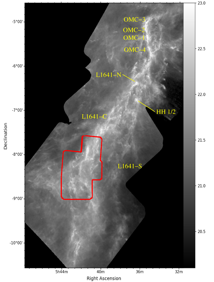
Fig. 2. As Fig. 1 for the Orion A giant molecular cloud, with the coverage of the ALCOHOLS survey in Orion A overplotted in red.
