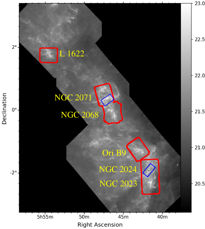
Fig. 1. Column density map ( \log N_{\text{H}} [\text{cm}^{-2}] ) towards the Orion B giant molecular cloud (greyscale; based on Herschel dust continuum mapping: Stutz & Kainulainen 2015; Stutz & Gould 2016; Stutz 2018) with the coverage of the ALCOHOLS survey in Orion B overplotted in red. The blue rectangles mark the coverage of the JCMT Legacy Survey of the Gould Belt in the NGC 2024 and NGC 2071 regions (Buckle et al. 2010).
