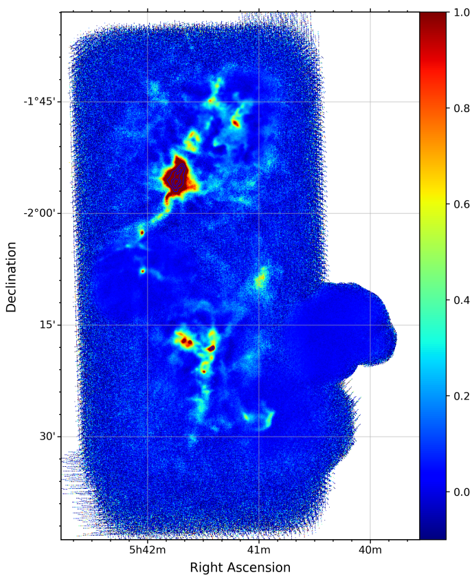
Fig. C.4. As Fig. C.1, for the NGC 2023/NGC 2024 area.
