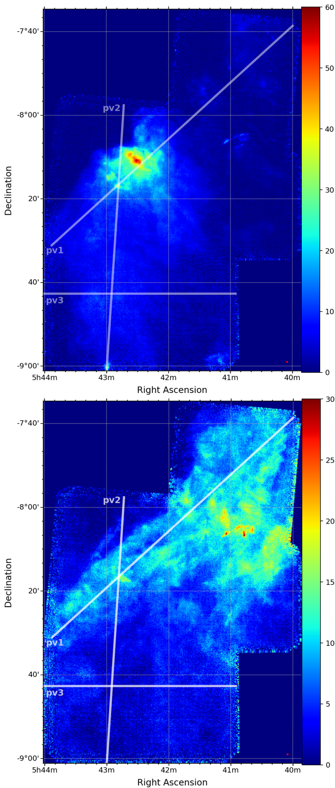
Fig. 31. CO emission in the L 1641-S field, integrated from 0.5 km/s to 3.5 km/s (top, in K km/s) and from 4.5 km/s to 7.25 km/s (bottom). The red dot in the bottom right corner indicates the beam size.
