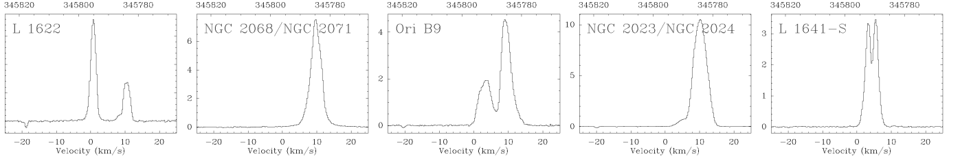
Fig. 6. CO spectra averaged over the full survey fields. L 1622 and Ori B9 each show two distinct velocity components, L1641-S also features a double peaked spectrum, while the NGC 2023, NGC 2024, NGC 2068, and NGC 2068 areas show single peaked spectra, though a hint of a secondary component is seen as a blue shoulder in the NGC 2023/NGC 2024 spectra.
