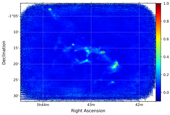
Fig. C.3. As Fig. C.1, for the Ori B9 area (combining own observations with the data presented by Miettinen et al. (2009)).
