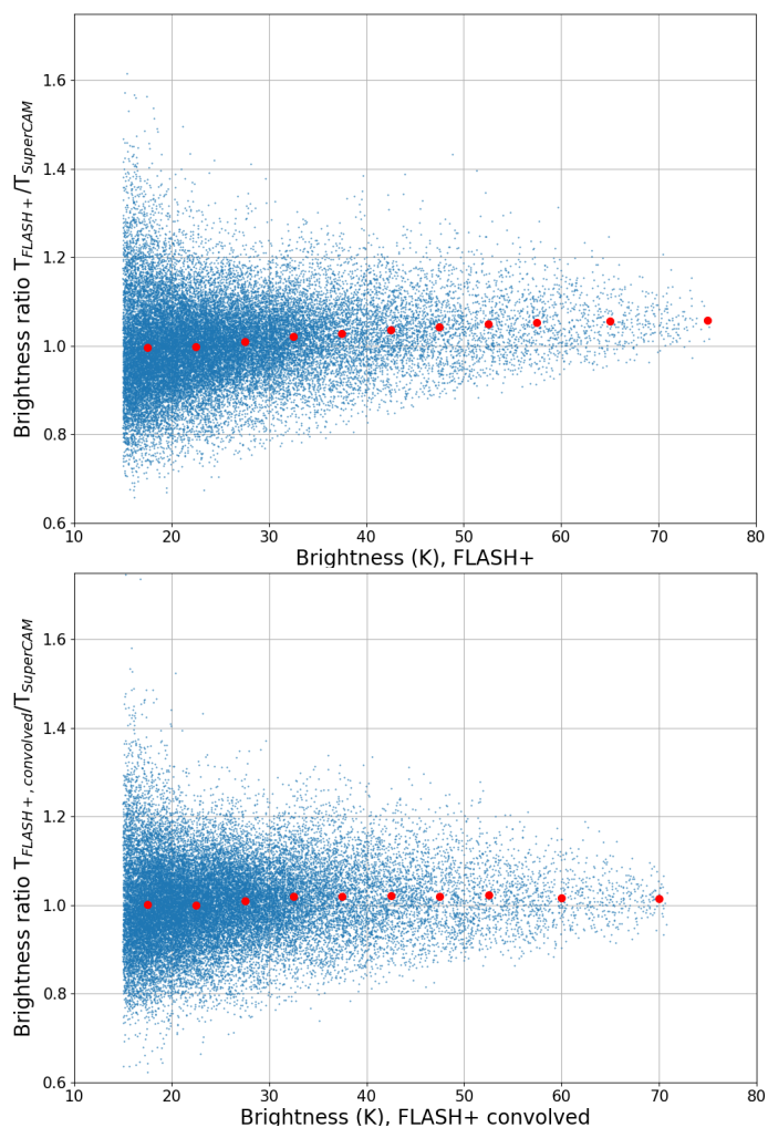
Fig. 4. Per pixel flux ratios (blue dots) of the Sandell et al. (2015) FLASH+ CO(3-2) NGC 2023 data to the ALCOHOLS SuperCAM data, as a function of the brightness of the FLASH+ data, for pixels with a FLASH+ brightness greater than 15 K. Red bullets represent flux ratios averaged over 5 K temperature bins (10 K bins for the two rightmost points). Top: direct ratio of the FLASH+ and SuperCAM data; bottom: ratio after convolving the FLASH+ data with a 9'' Gaussian.
