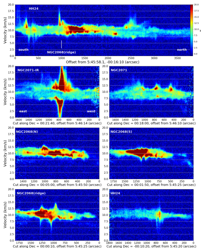
Fig. 12. Position velocity cuts across the NGC 2068/NGC 2071 survey field. Top: cut starting from 5:45:58.1, -0:16:10 (south-west), ending at 5^{\text{h}}47^{\text{m}}57^{\text{s}}.0 , +00^{\circ}39'10'' (north-east).
