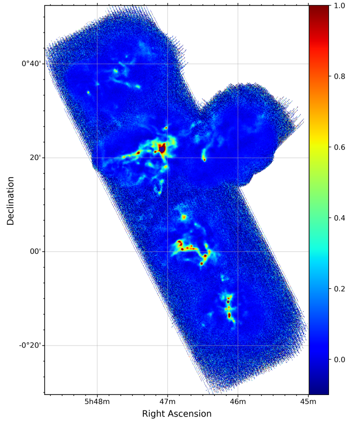
Fig. C.2. As Fig. C.1, for the NGC 2068/NGC 2071 field.
