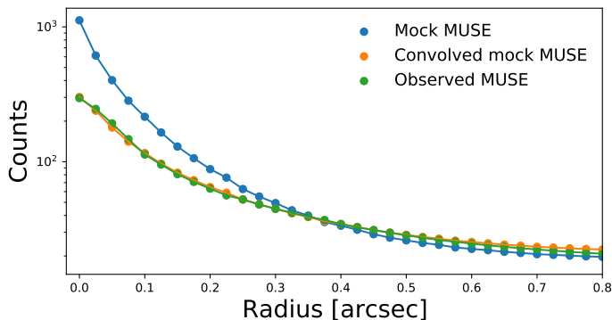
Fig. 3. The radial brightness profile of Nucleus 2 is shown for the unconvolved mock cube in blue, the mock cube convolved with the best-fit AO PSF at 7500Å shown in orange and the actual observed luminosity profile with MUSE is shown in green.
