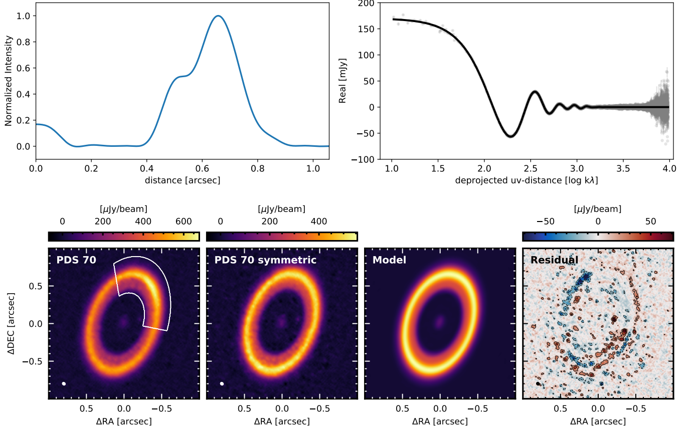
Figure 8. Results of the 1-D modelling of the disk, with the LB19+IB17+LB16 dataset. Upper left: best radial intensity profile obtained with the frank package. Upper right: observed visibilities (grey) compared to the best fit model (black). Bottom panels: Left: image of the LB19+IB17+LB16 continuum emission with the mask used to build the model for the asymmetry; Middle left: the resulting symmetric continuum emission after subtracting the asymmetry; Middle right: the best frank model; Right: the residual map. All images are obtained with a robust parameter of 0.5.
