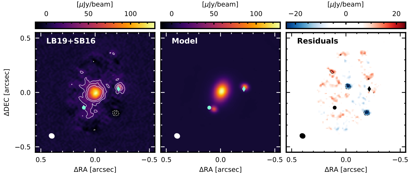
Figure 3. From left to right: Cavity image for LB19+SB16; Galarío best fit model for the inner disk, b_{\text{smm}} , and c_{\text{smm}} ; Residuals from the Galarío best fit model. All images are obtained with r=1 . Contours are 3, 6, 9 \sigma . Dashed contours correspond to -6, -3\sigma . The predicted positions of the two planets in July 2019 are indicated with a circle and diamond (PDS 70 b and c, respectively).
