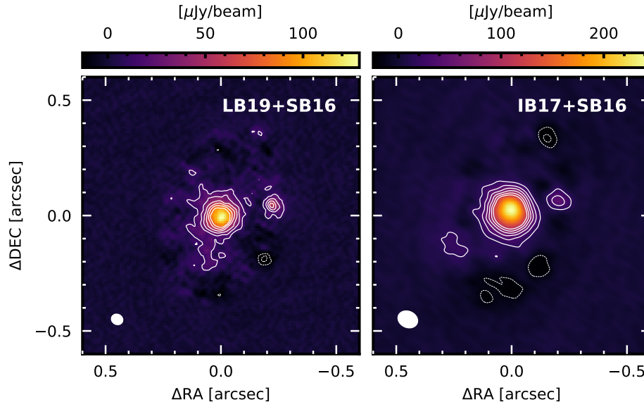
Figure 2. Residual images obtained after subtracting the Fourier transform of the CLEAN model for the outer ring (referred to as ‘cavity images’), obtained with the new data (LB19+SB16; left) and the data published in Isella et al. (2019) (IB17+SB16; right) considering a Briggs robust parameter of 1. Contours are 3 to 18 times the rms noise level ( 4.7 and 6 \mu\text{Jy beam}^{-1} , respectively), spaced in steps of 3\sigma . Dashed contours correspond to -3\sigma . A gallery of cavity images is given in Appendix A.2.
