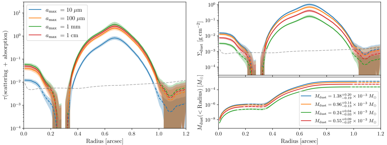
Figure 4. Left: Total optical depth of the continuum emission computed from the azimuthally averaged radial profile of the r=1 image of LB19+IB17+SB16. The lines show 4 models with different maximum grain sizes. The grey dashed line corresponds to a floor value of 3\sigma/\sqrt{N} , with \sigma the image rms, and N the number of beams in a radial bin. Shaded regions indicate error bars, computed as the square root of the quadratic sum of the image rms, the standard deviation in the radial bin and the 10% flux uncertainty. Right: dust surface density profiles (top) and corresponding cumulative masses (bottom).
