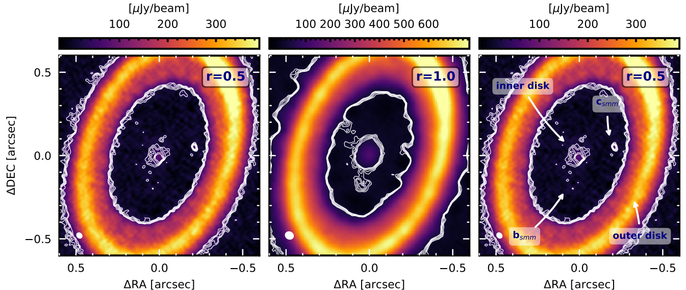
Figure 1. Images of the new continuum observations of PDS 70 (LB19+SB16). The data were imaged with a robust parameter of 0.5 (left) and 1 (center), with resolutions of 0.036'' \times 0.030'' and 0.051'' \times 0.044'' , respectively. The right panel shows the same image as in the left panel, with annotations. Beams are in the bottom left corner of each panel. Contours are 3 to 7\sigma , spaced by 1\sigma (with \sigma=8.8 and 4.8 \mu\text{Jy beam}^{-1} , respectively). An image gallery for all datasets is given in Appendix A.2.
