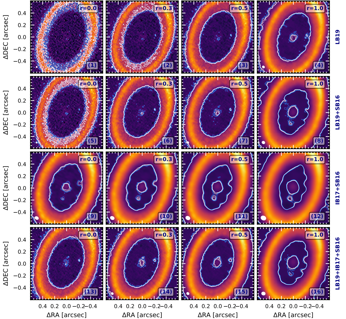
Figure 5. Gallery of images for all datasets. 3 and 4 \sigma contours and 5, 6, 7 \sigma contours are showed in blue and white, respectively. Rows correspond to different datasets, while columns are for different Briggs robust values (from 0 to 1; from left to right).
