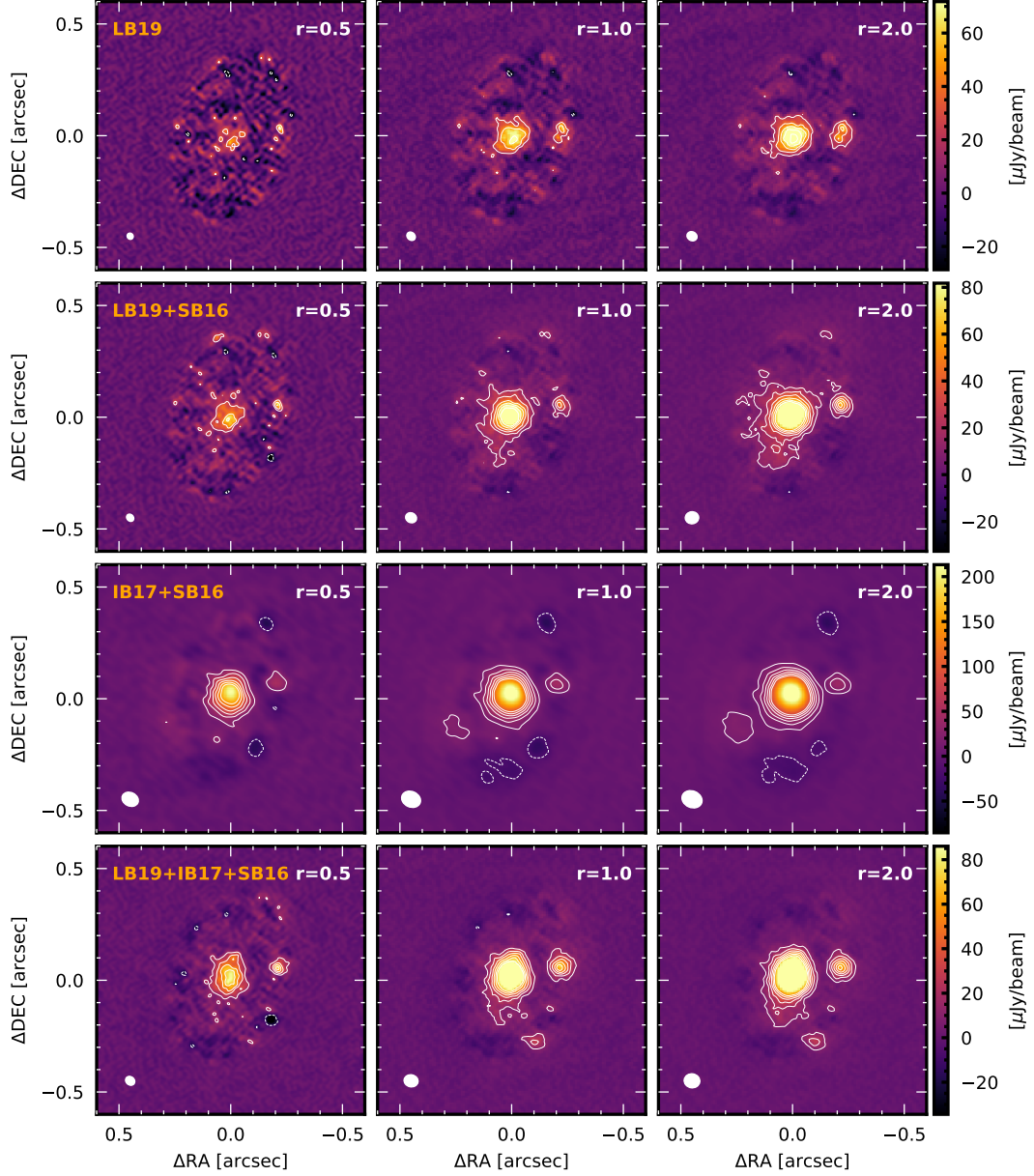
Figure 6. Gallery of cavity images. Contours are 3 to 18\sigma , spaced by 3\sigma . Dotted lines traces contours at -3\sigma . Rows correspond to different datasets, while columns are for different Briggs robust values (0.5, 1, 2, from left to right).
