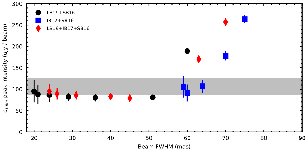
Figure 7. Peak intensity of c_{\text{smm}} as a function of angular resolution. The peak intensity of the CPD is constant around \sim 80 – 105 \mu\text{Jy beam}^{-1} when it is well separated from the outer ring. At larger resolution than \sim 60 mas, the peak intensity increases because the beam contains contribution from the outer disk. The grey area reports the estimate of Isella et al. (2019).
