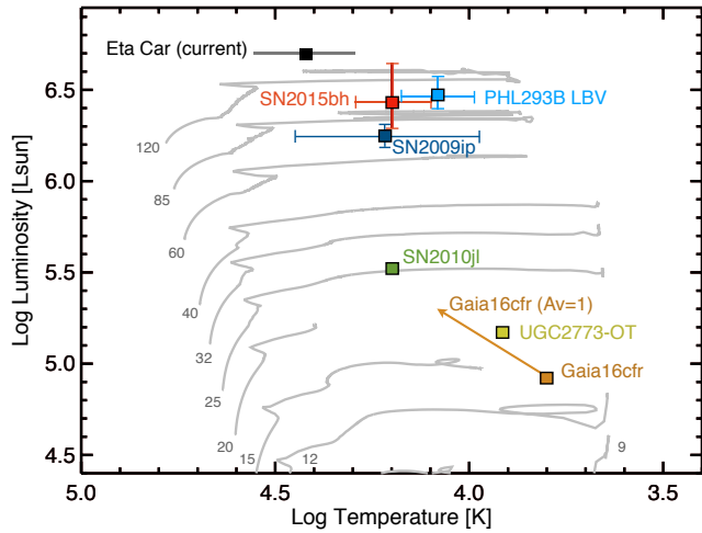
Figure 7. HR diagram showing the location of the LBV in PHL 293B during 2002–2011. We also include Eta Car (Groh et al. 2012b) and the progenitors of SN 2015bh (Boian & Groh 2018), SN 2009ip (Smith et al. 2010; Foley et al. 2011), UGC2773-OT (Smith et al. 2010), SN 2010jl (Smith et al. 2011), and Gaia16cfr (Kilpatrick et al. 2017). We also show in grey the evolutionary tracks for rotating stars with initial masses in the range 9 – 120 M_{\odot} at Z = 0.0004 (Groh et al. 2019b).
