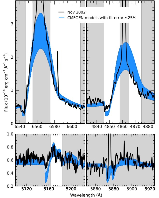
Figure 2. Comparison of the 2002 UVES spectrum of PHL 293B (black) to our best-fitting CMFGEN models. Blue region corresponds to models with a fit error \leq 25\% . White regions show the wavelength ranges considered in the fit. The upper left and right panels display the H- \alpha and H- \beta emission lines respectively. The lower left panel includes the tested Fe II 5169 Å emission line in addition to weaker Fe II 5159 Å and N I 5198 Å emission and Fe III 5156 Å absorption. Some best fit models also feature weak Mg I 5173 Å and 5184 Å and Tk II 5186 Å and 5189 Å. The lower right panel includes the He I 5786 Å line as well as Na I 5890 Å and 5896 Å emission.
