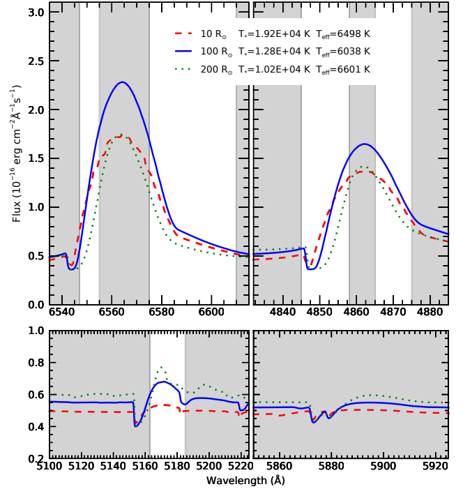
Figure 4. CMFGEN radiative transfer models for different stellar radii. The solid-blue spectrum belongs to one of our best fit models with the following parameters; R_* = 100 R_\odot , L_* = 2.52 \times 10^6 L_\odot and \dot{M} = 0.008 M_\odot \text{ yr}^{-1} . We compare this to two otherwise identical models but with R_* = 10 R_\odot (dashed red line) and R_* = 200 R_\odot (dotted green line).
