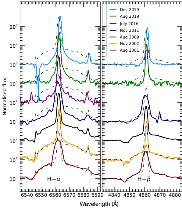
Figure 1. Spectroscopic evolution of PHL 293B between 2001 (lowest spectrum) and 2019 (highest). The 2009 X-shooter spectrum (dashed grey) is overlotted to all spectra, which are also shifted for clarity.
