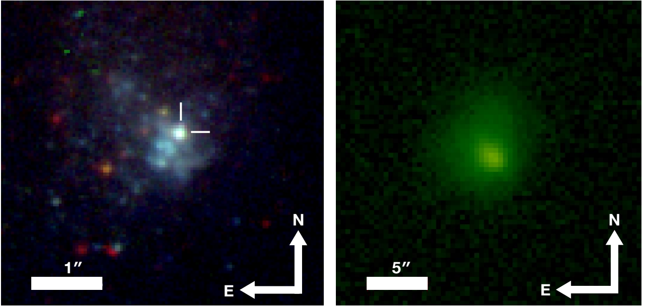
Figure 5. Left: High-spatial resolution colour-composite image of PHL obtained with HST WFC3 on 2010-10-31 (GO-12018; PI Prestwich). Right: SDSS g -band image of PHL 293B taken on 2003-10-24. The spatial scales are indicated by the horizontal bar.
