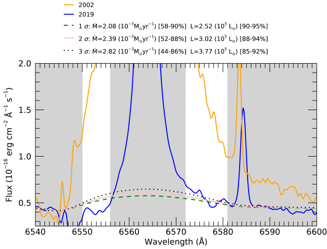
Figure 6. CMFGEN models compared to the 2019 X-shooter spectrum (blue). The models correspond to upper limits of L_{\text{surv}} and \dot{M}_{\text{surv}} with 1 (dashed green), 2 (solid pink), 3 (dotted black) \sigma confidence. The 2002 UVES spectrum (yellow) is included to highlight the significant reduction in the broad H- \alpha emission.
