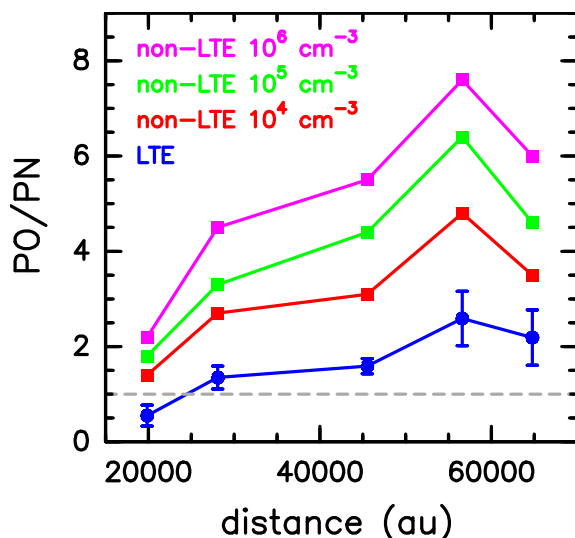
Figure 12. PO/PN molecular ratio, normalized to the ratio found in the P2 spot, as a function of the distance to the central MM position. We have included all the P-spots of the southern cavity, with the exception of the P7 spot, because it is located very close to the primary beam of the observations, where poorer sensitivity may affect the accuracy of the measured PO column density. The different colors indicate the molecular ratios obtained with the LTE approximation (blue dots) and the non-LTE analysis considering different densities: 10^4 \text{ cm}^{-3} (red squares), 10^5 \text{ cm}^{-3} (green squares), and 10^6 \text{ cm}^{-3} (magenta squares).
