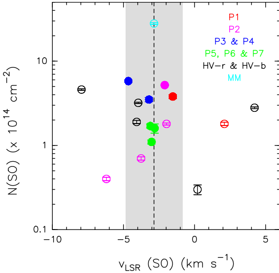
Figure 7. SO column density versus SO velocity towards the different positions in the AFGL5142 field studied in this work. The filled/empty circles indicates detections/non-detections of PN. The different colors denote different group of positions, as labeled in the upper right corner. The uncertainties on the column densities are indicated with error bars. The uncertainties on the velocities are within the size of the symbols. The systemic velocity of the central core, -2.85 km s ^{-1} , is indicated with a vertical dashed line. The gray band indicates a velocity range of \pm 2 km s ^{-1} with respect to the systemic velocity, which contains all the regions with PN detections.
