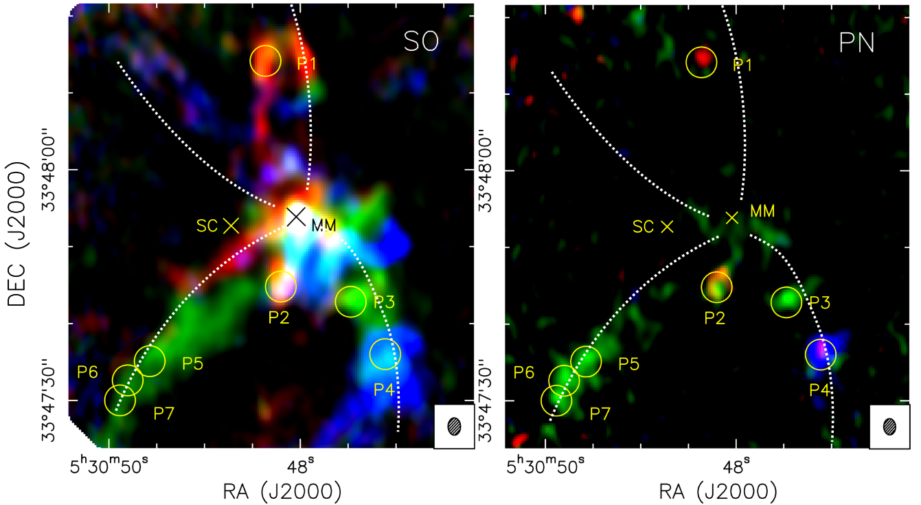
Figure 2. ALMA integrated maps of SO( 2_3-1_2 ) (left) and PN( 2-1 ) (right) in three velocity ranges [-6.5,-4.5] km s ^{-1} (blue); [-4.5,-2.0] km s ^{-1} (green); [-2.0, 0] km s ^{-1} (red). The cavity of the bipolar outflow is indicated with dashed white curves. The positions of the starless core (SC) and the MM core are indicated with yellow (or black) crosses. The different P-spots (P1–P7) are identified with yellow circles. The beams of the observations are indicated in the lower right corner of each panel.
