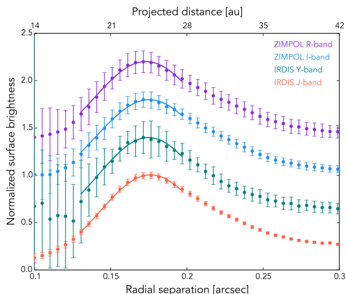
Fig. B.1. Azimuthally averaged polarized surface brightness around the cavity edge of the outer disk. The profiles are shown in normalized units and with arbitrary offsets. The data points show the mean Q_\phi value in each bin and the error bars show 1\sigma deviations in the corresponding U_\phi bin. Solid lines show the best-fit Gaussian profiles (see also Table B.1).
