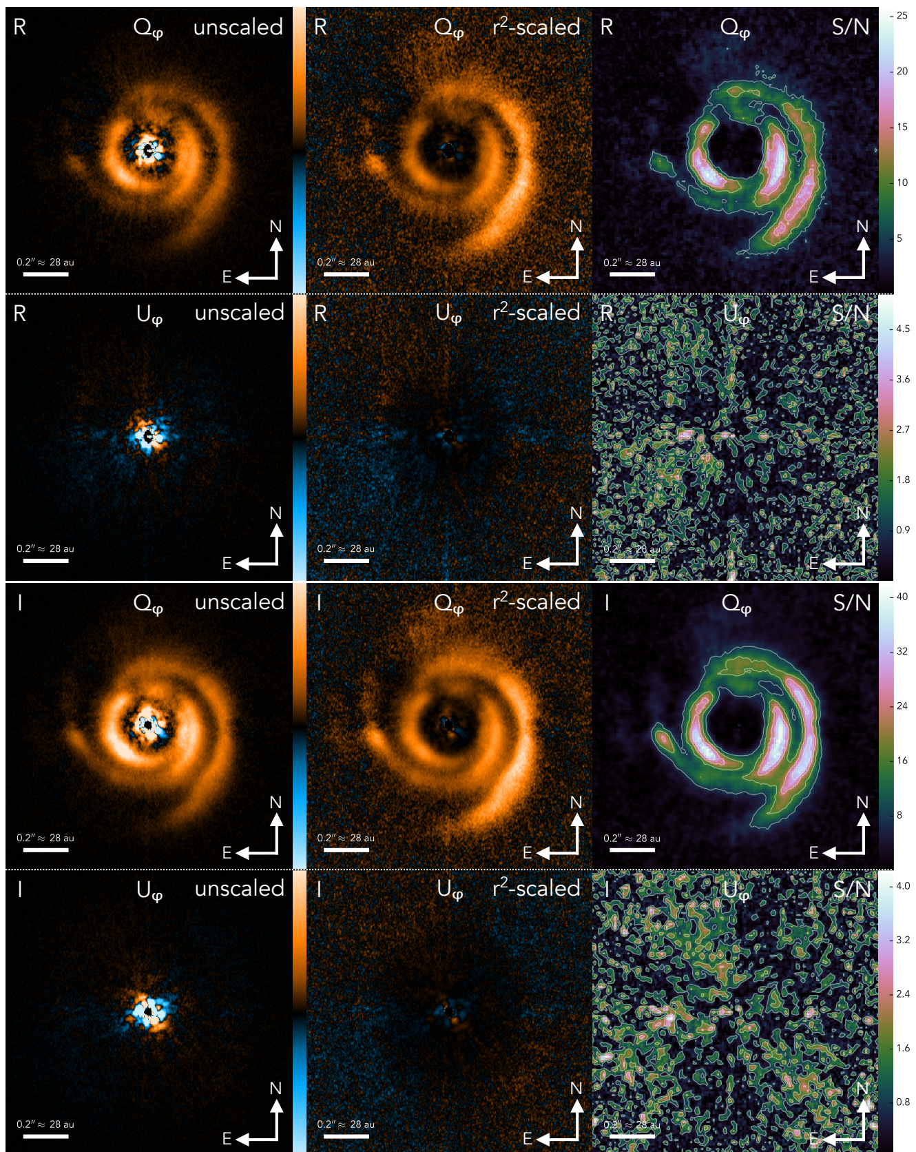
Fig. 1. ZIMPOL R -band (top two rows) and ZIMPOL I -band (bottom two rows) polarized intensity images. The field of view is 1''.4 \times 1''.4 and the central star is positioned in the center of each image. The left column shows the Q_\phi and U_\phi polarized intensity images (see Sect. 2.3). The center column shows the Q_\phi and U_\phi images scaled with the deprojected distance squared from the star to each pixel for an inclination of 11^\circ and a position angle of the major axis of 62^\circ . All images are shown on a linear color stretch, with companion Q_\phi and U_\phi images having the same minimum and maximum value. Orange corresponds to positive values, blue to negative values, and black is the zero point. The right column shows the signal-to-noise (S/N) maps of the Q_\phi and U_\phi images which are obtained from the U_\phi images. The contour levels correspond to the standard deviation values that are shown on the right of the S/N map colorbar.
