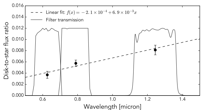
Fig. 5. Disk-to-star flux ratio as determined from the Q_\phi image, which only includes polarized scattered light from the disk, and an unsaturated total intensity image, which is dominated by the stellar halo. The three data points are the flux ratios in R -, I -, and J -band with 3\sigma error bars. The dashed line shows a weighted least squares fit of a linear function and the solid lines are the normalized transmission curves of the three filters.
