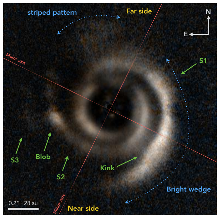
Fig. 4. Color composite RGB image of ZIMPOL R -band (blue), ZIMPOL I -band (red), and the average of R - and I -band (green). The field of view is 1''.4 \times 1''.4 and the main features that have been identified are labeled.
