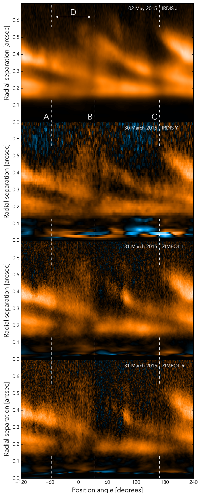
Fig. 7. Polar projections of the r^2 -scaled Q_\phi images for J -, Y -, I -, and R -band (top to bottom). The vertically dashed lines correspond to shadow lanes A, B, and C and are identical to the dashed lines in Fig. 8. The identified shadow features have been labeled in the J -band image. North corresponds to PA = 0^\circ and positive position angles are measured east from north.
