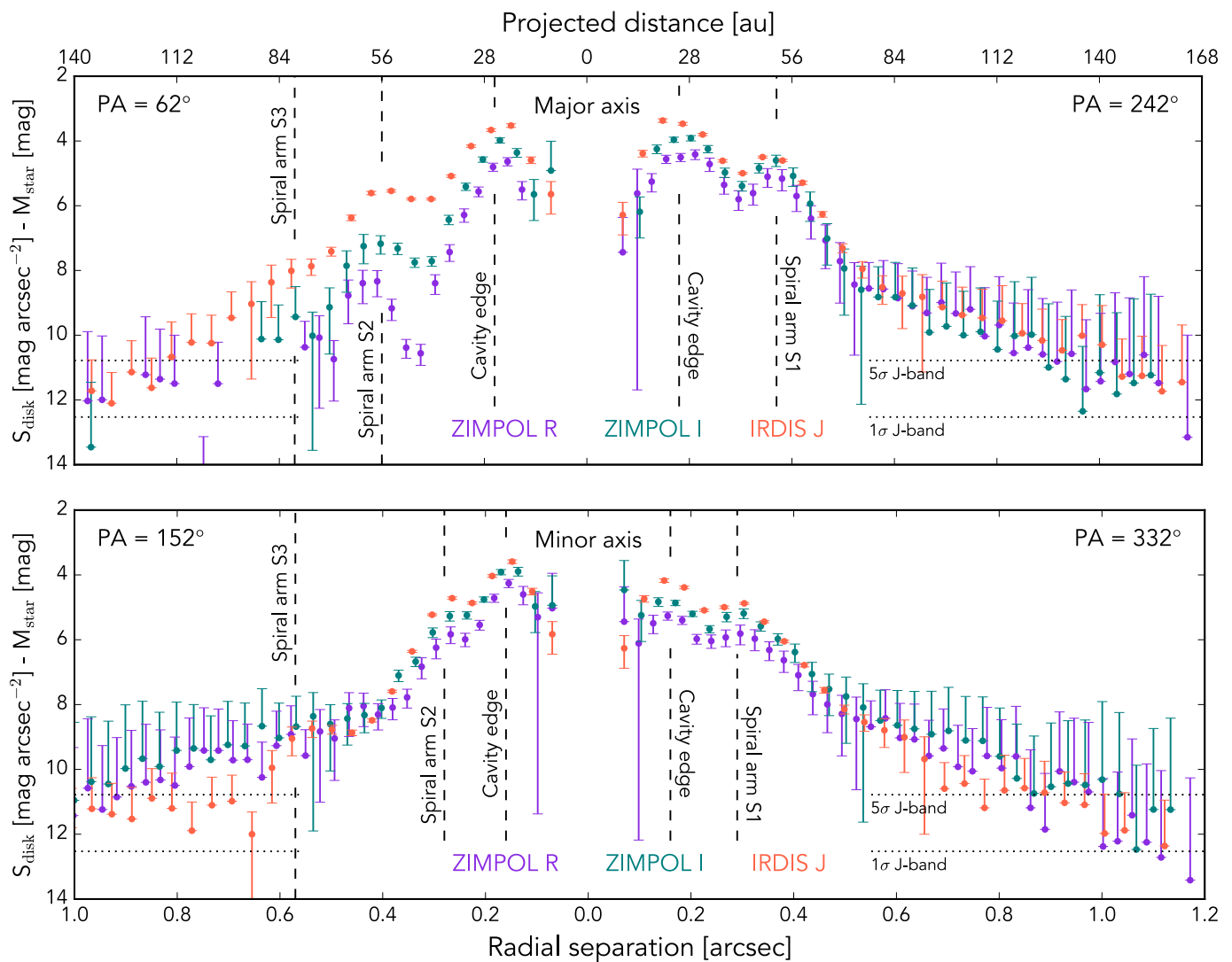
Fig. 6. Polarized surface brightness profiles along the major axis (top) and minor axis (bottom) of the HD 135344B disk. The position angle of the axis (measured east of north) is shown in the top left/right and the colors indicate different filters. Data points show the mean Q_\phi surface brightness and the error bars show 1\sigma uncertainties determined from the corresponding U_\phi image. We have rejected bins in which the mean Q_\phi count rate is negative as well as lower limit error bars that correspond to negative flux values. We note that the error bars do not include the uncertainty from the photometric calibration. The dotted lines show 1\sigma and 5\sigma background levels in the Q_\phi J -band image at large separation from the star.
