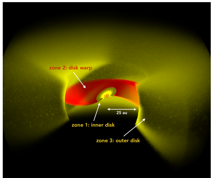
Fig. 9. Architecture of the MCMMax3D radiative transfer model (exaggerated for clarification of the disk warp). The misaligned inner disk (zone 1) and outer disk (zone 3) are shown in yellow. The warped disk region (zone 2), which transitions the orientation of the inner disk towards the outer disk, is shown in red.
