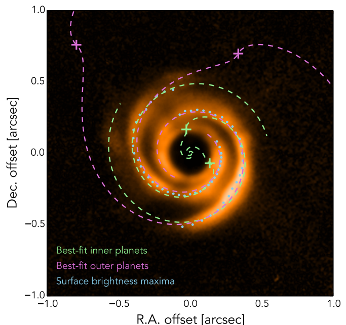
Fig. 10. Best-fit spiral arm solutions for the protoplanets inside (green) and outside (purple) the scattered light cavity (see also Table 4). Blue points are the surface brightness maxima along each spiral arm that are used for the \chi^2 fitting. The plus symbols indicate the positions of the best-fit protoplanets.
