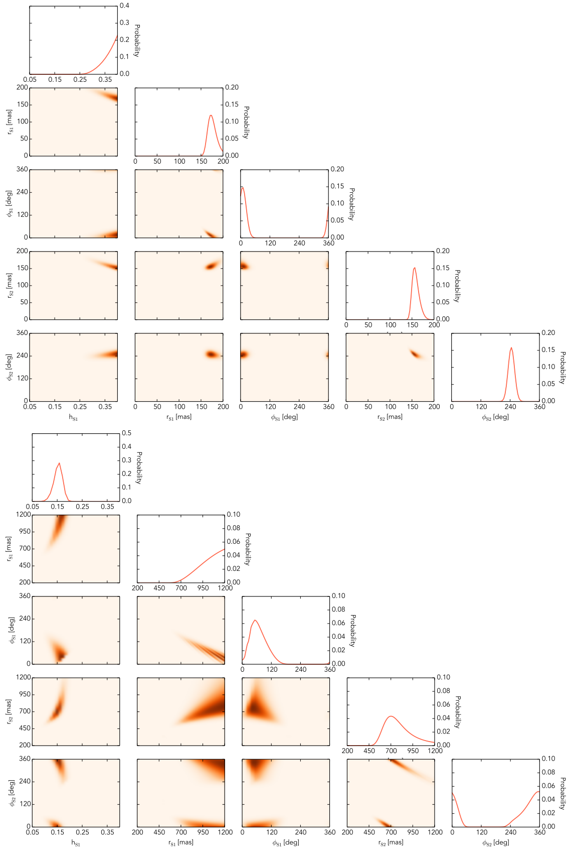
Fig. C.1. Bayesian probabilities for the simultaneous fit of spiral arms S1 and S2 (see Fig. 4). The protoplanet locations have been restricted to either inside (top triangle diagram) or outside the scattered light cavity (bottom triangle diagram). The exponent of the sound speed profile is kept fixed to \eta = 0.25 . The colored maps are the 2D probabilities of each set of free parameters and the top row of each column shows the marginalized probabilities of the free parameters that were fitted.
