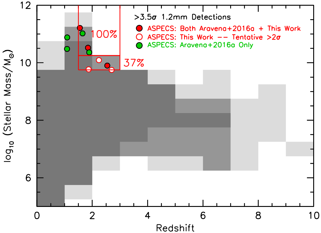
FIG. 6.— Stellar mass vs. redshift range covered by sources identified over the \sim 1 arcmin 2 ASPECS region, with light, medium dark, and dark gray indicating regions where \geq 1 , \geq 3 , and \geq 7 sources are found (where each region subtends \Delta M \sim 0.5 dex \times \Delta z \sim 1 ). Large filled red circles indicate those sources where continuum detections ( >3.5\sigma ) are found in both present study + paper II of the ASPECS series (Aravena et al. 2016a). Green circles indicate sources that are only found in paper II of ASPECS (Aravena et al. 2016a). Open red circles indicate those galaxies which show tentative >2\sigma detections in ASPECS. 100% and 37% of the star-forming z = 1.5 - 3.0 sources in the stellar mass range \log_{10} M/M_{\odot} > 10.25 and 9.75 - 10.25 (indicated with the red boxes), respectively, show detections in the ALMA continuum 1.2 mm data. It is clear that stellar mass is an especially useful predictor of IR luminosity over a wide range in redshift. Inspiration for this figure came in part from Figure 6 of Dunlop et al. (2016).
