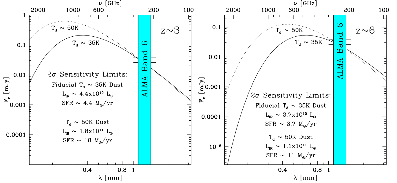
FIG. 1.— Model SEDs in the far IR for the faintest z \sim 3 and z \sim 6 galaxies we would be able to obtain tentative individual detections ( > 2\sigma ) in our deep ALMA band-6 observations. The plotted SED are modified blackbody SEDs with a dust temperature of 35 K and a dust emissivity power-law spectral index of \beta_d = 1.6 (Eales et al. 1989; Klaas et al. 1997). The two short horizontal lines at 1.2mm show our 2\sigma and 3\sigma sensitivity limits. At both z \sim 3 and z \sim 6 , we would expect to tentatively detect individual galaxies to approximately the same IR luminosity \sim 4 \times 10^{10} L_\odot , which is equivalent to an obscured star-formation rate (SFR) of \sim 4 M_\odot/\text{yr} . For galaxies with dust temperatures of 50 K, we would expect to tentatively galaxies to a IR luminosity \sim 1.8 \times 10^{11} L_\odot and \sim 1.1 \times 10^{11} L_\odot at z \sim 3 and z \sim 6 , equivalent to obscured SFRs of \sim 18 and \sim 11 M_\odot/\text{yr} , respectively. These sensitivities account for the impact of the CMB (da Cunha et al. 2013).
