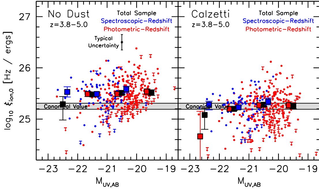
FIG. 17.— ( left ) New estimates of the Lyman-continuum photon production efficiencies \xi_{ion} in z = 4-5 galaxies (following Bouwens et al. 2015) using IRAC-based H\alpha luminosities and HST-based UV luminosities. Sources where spectroscopic redshifts or well-determined photometric redshifts place the H\alpha line in a specific IRAC band are indicated by the blue and red points, respectively. 1\sigma upper limits are included on this diagram with downward arrows in cases where the H\alpha emission line is not detected at 1\sigma in the photometry. The solid red and blue squares indicate the mean value of \xi_{ion} for red and blue colored points, while the solid black square indicate the mean values combining the spectroscopic and photometric-redshift selected samples. The grey band indicates the Lyman-continuum photon production efficiencies \xi_{ion} assumed in typical models (e.g., Madau et al. 1999; Kuhlen & Faucher-Giguère 2012; Robertson et al. 2013). The black error bar near the top of the left panel indicate the typical uncertainties in the derived \xi_{ion} 's. ( right ) Estimated Lyman-continuum photon production efficiencies \xi_{ion} if a Calzetti extinction law is assumed. The derived values are \sim 0.24 dex lower and were previously presented by Bouwens et al. (2015). If dust extinction is as low in z \sim 4-5 galaxies as suggested using our fiducial T_d \sim 35 K results, it would imply that z \sim 4-5 galaxies produce up to \sim 1.8\times as many ionizing photons per unit UV luminosity as expected in conventional models.
