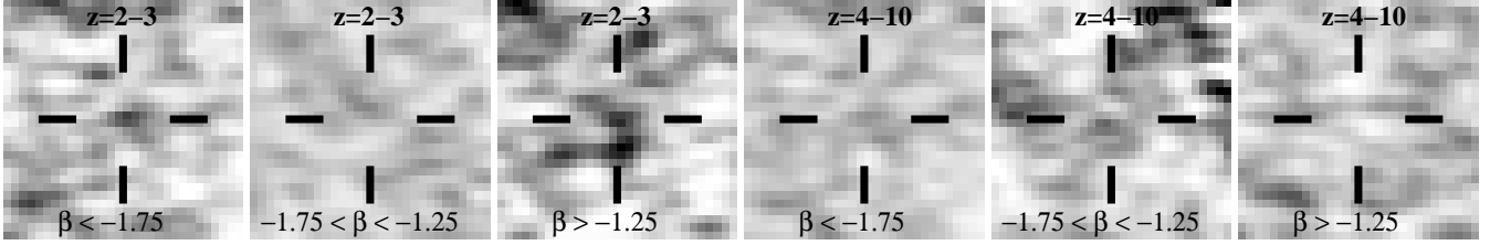
FIG. 11.— Stacked 1.2 mm-continuum images ( 9'' \times 9'' ) for z = 2-3 and z = 4-10 galaxies falling in different bins of UV -continuum slope \beta . All sources that are individually detected at \geq 4\sigma are not included in the presented stack results. Only the most massive ( > 10^{9.75} M_{\odot} ) sources are included in our z = 2-3 stacks, while our z = 4-10 stacks include sources over the full mass range (due to the small number of sources with > 10^{9.75} M_{\odot} ). In the stacks, sources are weighted according to the expected 1.2 mm-continuum flux (assuming L_{IR} \propto L_{UV} ) and according to the inverse square of the noise. The 3 individually-detected sources (at > 4\sigma ) are not included in the presented stack results.
