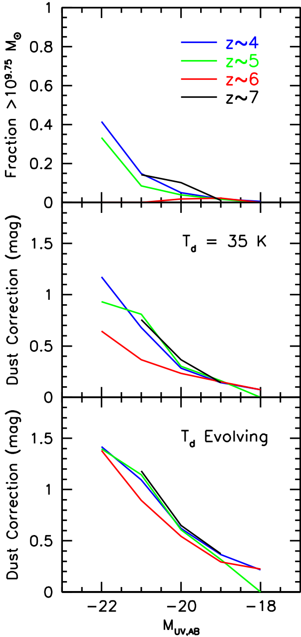
FIG. 14.— (upper panel) Fraction of z \sim 4 (blue line), z \sim 5 (green line), z \sim 6 (red line), and z \sim 7 (black line) galaxies (red line) in a given 0.5-mag bin of UV luminosity estimated to have a stellar mass in excess of 10^{9.75} M_{\odot} where the dust extinction appears to be especially significant. (middle panel) Estimated correction for dust extinction versus UV luminosity for z \sim 4 (blue), z \sim 5 (green line), z \sim 6 (red line), and z \sim 7 (black line). For sources with stellar masses in excess of 10^{9.75} M_{\odot} , dust extinction is computed using the M99 IRX- \beta relation, while for those with stellar masses lower than 10^{9.75} M_{\odot} , dust extinction is computed based on the consensus z \sim 2-3 IRX-stellar mass relation (but shifted lower by 0.5 dex). (lower panel) Similar to middle panel, but computing dust extinction for the lowest-mass galaxies assuming no evolution in the IRX-stellar mass relation from z \sim 0-3 (appropriate if the dust temperature monotonically increases to high redshifts). See Figure 13.
