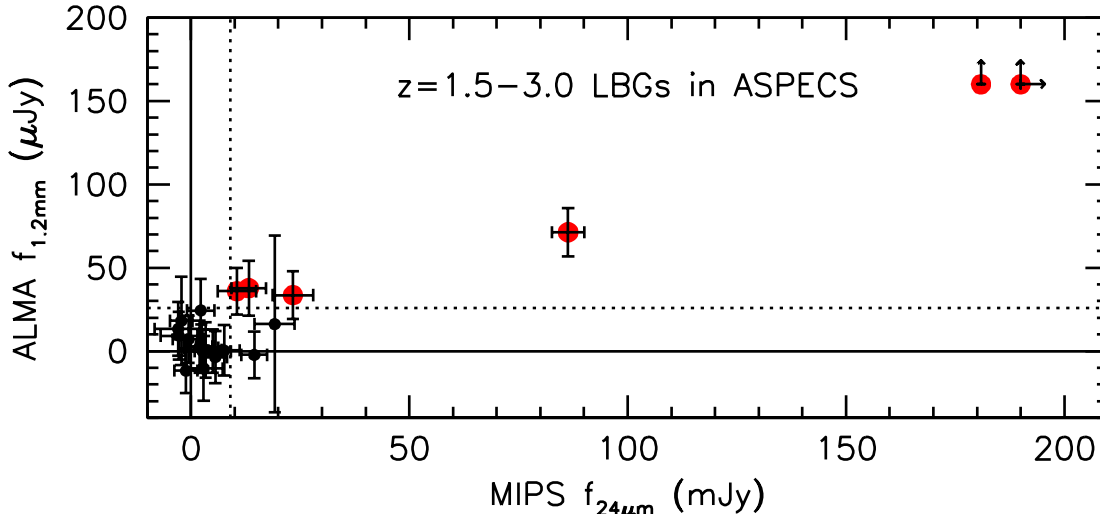
FIG. 19.— Comparison of the observed MIPS 24\mu\text{m} fluxes (Whitaker et al. 2014) for sources in our z \sim 1.5\text{--}3.0 LBG sample with the 1.2\text{ mm} continuum fluxes measured from ASPECS (solid black circles with 1\sigma error bars shown). The larger solid red circles correspond to the sources we claim detections or tentative ALMA 1.2\text{ mm} detections. The arrows indicate that the measured fluxes lie outside the bounds of the figure. The horizontal and vertical dotted lines show the approximate flux levels where 2\sigma detections are expected. The MIPS 24\mu\text{m} fluxes exhibit a broad correlation with the ALMA 1.2\text{ mm} fluxes for z \sim 1.5\text{--}3.0 galaxies, and those sources which are detected at >2\sigma in the ALMA observations also tend to show significant >2\sigma detections in the MIPS observations (see Table 10).
