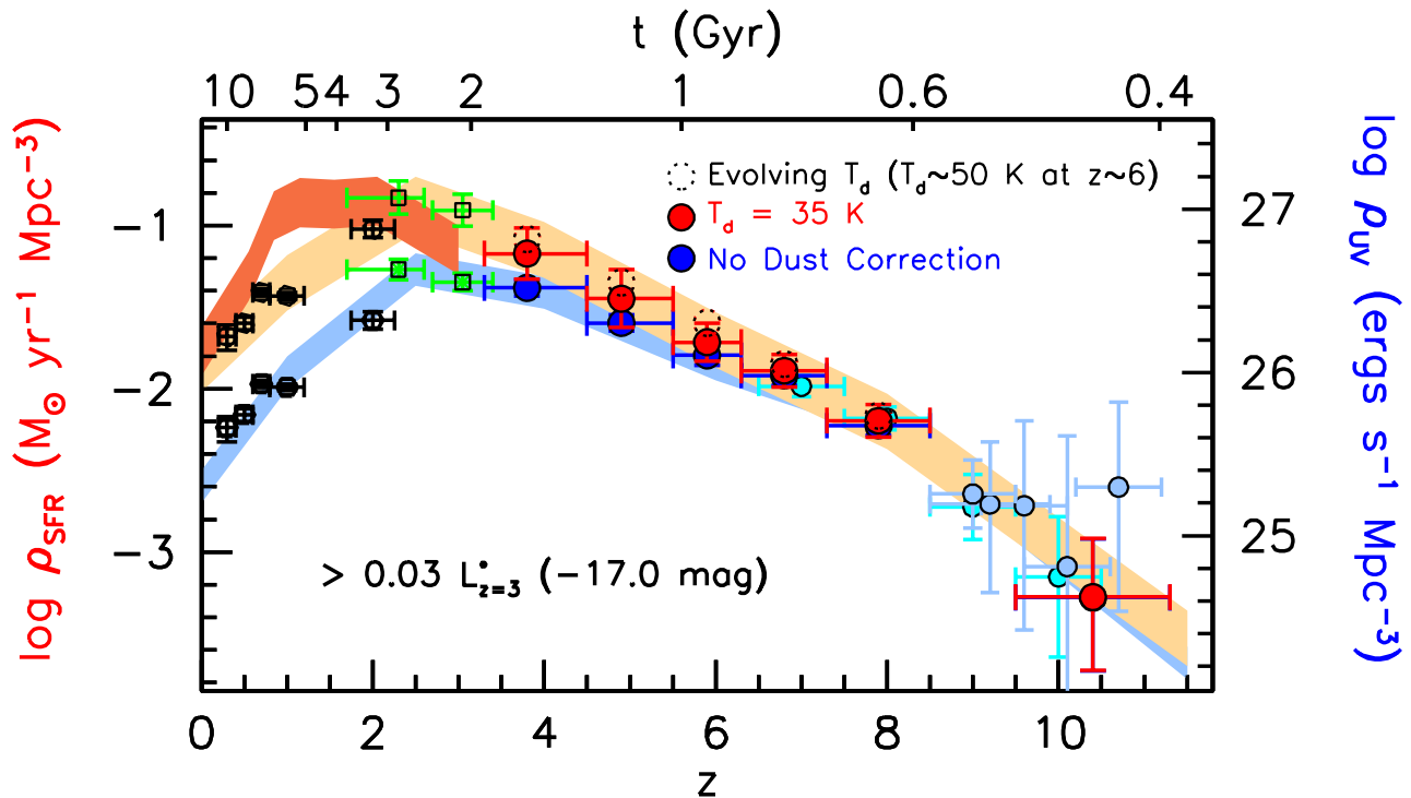
FIG. 15.— Updated determinations of the derived SFR ( left axis ) and UV luminosity ( right axis ) densities versus redshift (§5.4). The left axis gives the SFR densities we would infer from the measured luminosity densities, assuming the Madau et al. (1998) conversion factor relevant for star-forming galaxies with ages of \gtrsim 10^8 yr (see also Kennicutt 1998). The right axis gives the UV luminosities we infer integrating the present and published LFs to a faint-end limit of -17 mag ( 0.03 L_{z=3}^* ) – which is the approximate limit we can probe to z \sim 8 in our deepest data set. The upper and lower set of points ( red and blue circles, respectively ) and shaded regions show the SFR and UV luminosity densities corrected and uncorrected for the effects of dust extinction. The dust correction we utilize relies on an IRX- \beta relation intermediate between SMC and Calzetti for the highest mass galaxies in the present samples, i.e., > 10^{9.75} M_{\odot} , but an IRX-stellar mass relation for lower-mass sources (§4.2). The dotted black open circles indicate the dust-corrected SFR densities, assuming an unevolving IRX-stellar mass relation (appropriate if the dust temperature increases monotonically towards high redshift: see Figure 13). The dark red shaded region include the contribution from IR bright sources (Magnelli et al. 2009, 2011, 2013). Also shown are the SFR densities at z \sim 2-3 from Reddy et al. (2009: green crosses ), at z \sim 0-2 from Schiminovich et al. (2005: black hexagons ), at z \sim 7-9 from McLure et al. (2013) and Ellis et al. 2013: cyan solid circles ), and z \sim 9-11 from CLASH (Bouwens et al. 2014b; Coe et al. 2013; Zheng et al. 2012: light blue circles ) and Oesch et al. (2013: light blue circles ). The z \sim 9-11 constraints on the UV luminosity density have been adjusted upwards to a limiting magnitude of -17.0 mag assuming a faint-end slope \alpha of -2.0 (consistent with our constraints on \alpha at both z \sim 7 and at z \sim 8 ).
