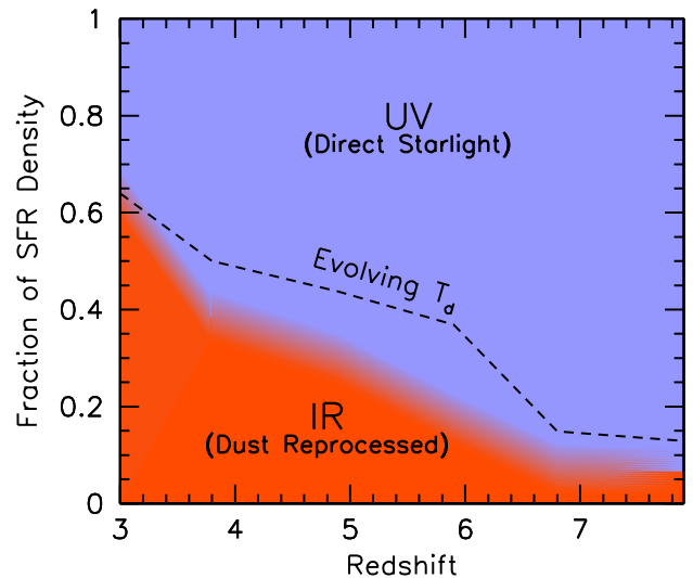
FIG. 16.— Fraction of the SFR density that would be directly observed in the IR and in the rest-frame UV according to our fiducial SFR density estimates (Table 8). The dashed line gives the dividing line for our fiducial evolving T_d scenario ( 35 \text{ K} \times ((1+z)/2.5)^{0.32} ; see §3.1.3). The present figure represents an update to Figure 12 from Bouwens et al. (2009). Similar to the conclusions from Bouwens et al. (2009), we find that most of the SFR density at z \gtrsim 3.5 appears to be directly observable in the rest-frame UV (see also Burgarella et al. 2013; Dunlop et al. 2016; Bourne et al. 2016).
