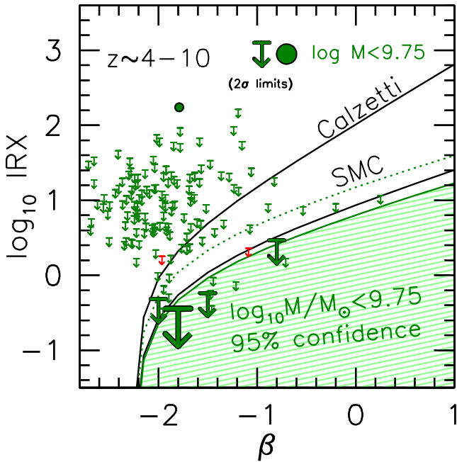
FIG. 12.— Stacked constraints on the infrared excess in z = 4-10 galaxies versus \beta . Similar to Figure 10 but for galaxies in the redshift range z = 4-10 . We only present results for the lower-mass subsample, as we find only 2 > 10^{9.75} M_{\odot} galaxies over the 1 arcmin 2 ASPECS region and those 2 sources are not detected. Our stack results (indicated by the larger downward-pointing arrows which express the 2\sigma upper limits) strongly suggest that the infrared excess for the typical lower-mass < 10^{9.75} M_{\odot} galaxy is low, even below that expected for an SMC dust law. The very large downward pointing arrow is as in Figure 10, but for z = 4-10 galaxies. The light-green-shaded region gives our derived constraints (95% confidence intervals) on the IRX - \beta relationship for z = 4-10 galaxies with all but the highest stellar masses ( < 10^{9.75} M_{\odot} ). The dotted green line indicates the upper bound on this region, if the dust temperature is much higher at z = 4-10 than at z \sim 1.5 (i.e., 44-50 K as suggested by the results of Bethermin et al. 2015).
