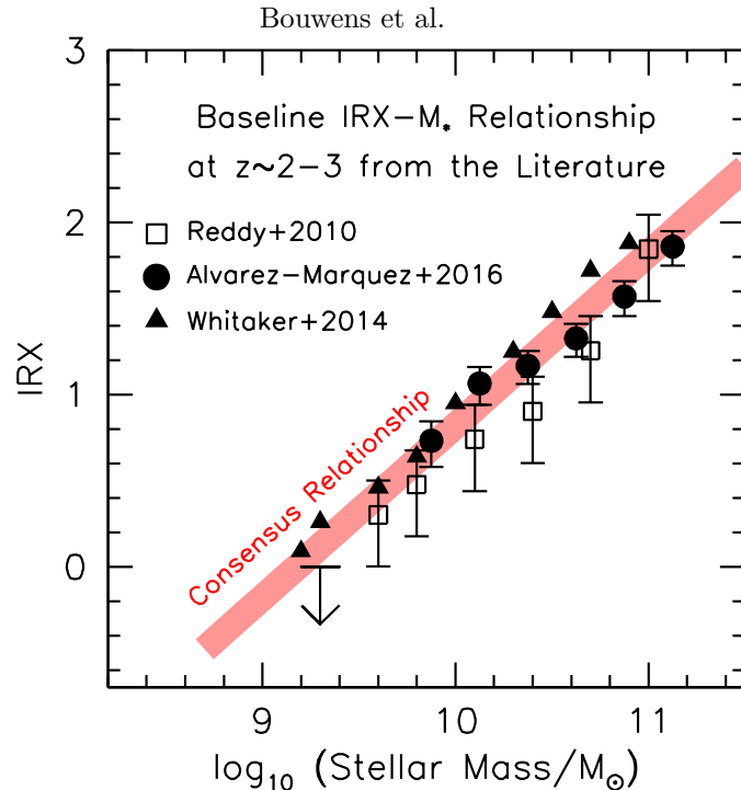
FIG. 18.— Consensus relationship between the infrared excess of galaxies and their stellar mass at z \sim 2-3 . The solid circles, open squares, and solid triangles show the results from Álvarez-Márquez et al. (2016), Reddy et al. (2010), and Whitaker et al. (2014). The thick light red line show the consensus relationship (Appendix A).
