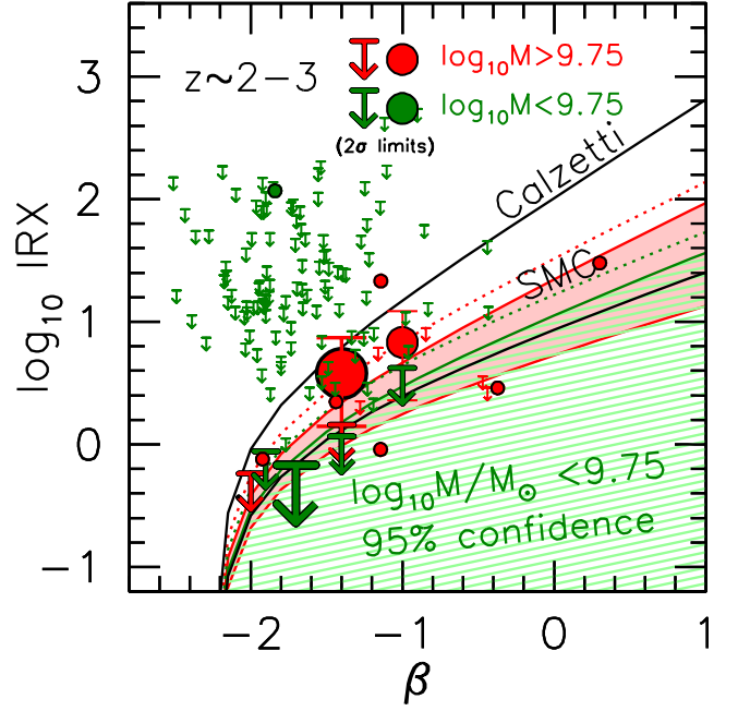
FIG. 10.— Stacked constraints on the infrared excess in z = 2-3 galaxies versus the UV -continuum slope \beta . These results are shown for higher- and lower-mass subsamples ( > 10^{9.75} M_\odot and < 10^{9.75} M_\odot ) of z = 2-3 galaxies (red and green solid circles and downward arrows, respectively) and were obtained by stacking the ALMA 1.2 mm observations of individual sources over the ASPECS region (excluding the one source XDFU-2397246112 with an AGN, but not excluding any other sources). Upper limits and errorbars are 2\sigma and 1\sigma , respectively. The smaller solid circles and downward arrows indicate a > 2\sigma measurement of the infrared excess and 2\sigma upper limits on this excess. The purpose of the smaller points is to show the constraints that can be derived from individual sources before stacking. The very large red circle and downward-pointing green arrow gives the value and 2\sigma upper limit, respectively, on IRX based on all > 10^{9.75} M_\odot and < 10^{9.75} M_\odot z = 2-3 sources from ASPECS plotted at the weighted value of \beta contributing the most signal to this measurement of IRX. The solid lines show the nominal IRX- \beta relation one would derive based on the Calzetti and SMC dust laws. The shaded red and light green regions indicate the 68% and 95% confidence intervals we can derive on the IRX- \beta relationship on the basis of our results for sources with stellar masses of > 10^{9.75} M_\odot and < 10^{9.75} M_\odot , respectively. If the dust temperature increases towards high redshift as indicated by Bethermin et al. (2015), the upper bound on these regions would be given by the dotted red and green regions. Our results are consistent with the IR emission from high-mass ( > 10^{9.75} M_\odot ) z \sim 2-3 galaxies exhibiting an SMC IRX- \beta relation. However, for lower-mass ( < 10^{9.75} M_\odot ) galaxies, our results suggest lower infrared excesses, less even than expected for an SMC dust law.
