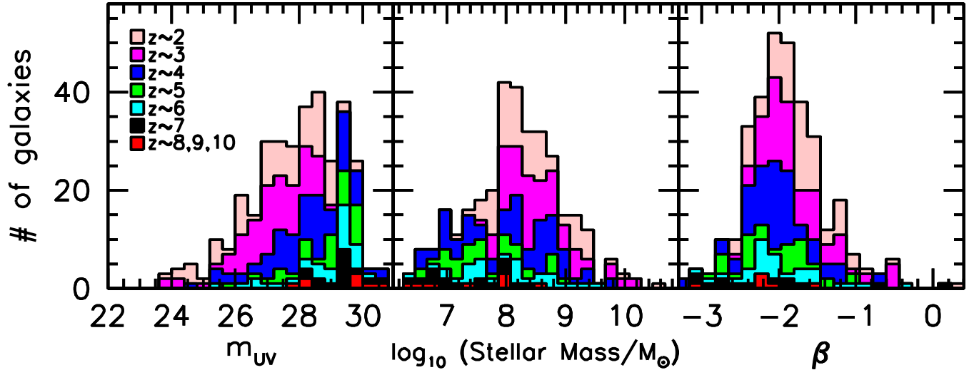
FIG. 2.— Cumulative histograms showing the composition of the HUDF z \sim 2 , z \sim 3 , z \sim 4 , z \sim 5 , z \sim 6 , z \sim 7 , and z \sim 8-10 samples we consider here (pink, magenta, blue, green, cyan, black, and red shaded histograms, respectively) as a function of apparent magnitude (measured at wavelengths probing the UV continuum), stellar mass, and UV-continuum slope \beta (left, central, and right panels, respectively). The deep far-IR continuum observations ( 12.7\mu\text{Jy}/\text{beam} RMS) from ASPECS make it possible for us to set the best constraints on the average dust emission from ( m_{UV} > 25 , < 10^{10} M_{\odot} ) galaxies thus far.
