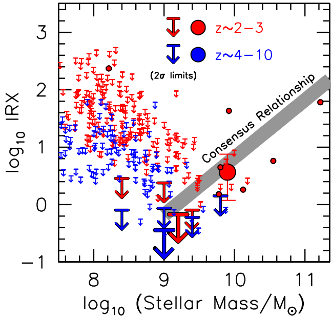
FIG. 8.— Constraints on the infrared excess of z = 2-3 and z = 4-10 galaxies (large red and blue circles and downward arrows, respectively) obtained by stacking the ALMA 1.2 mm observations available for many individual sources over the 1 arcmin 2 ASPECS region (excluding the one source XDFU-2397246112 with an AGN, but not excluding any other sources). The small filled circles and downward arrows are for sources with a positive 2\sigma measurement of IRX and 2\sigma upper limit on IRX, respectively. Upper limits and errorbars are 2\sigma and 1\sigma , respectively. A redshift-independent dust temperature of 35 K is assumed in deriving these results. The presented upper limits on our z = 4-10 sample would be 0.4 dex higher if the dust temperature in higher-redshift galaxies is significantly higher than at z \sim 1.5 (i.e., 44-50 K as suggested by the results of Magdis et al. 2012 and Bethermin et al. 2015). The thick-shaded grey line shows the consensus dependence of IRX on galaxy stellar mass we derive for z \sim 2-3 galaxies (Appendix A) from the literature (Reddy et al. 2010; Whitaker et al. 2014; Álvarez-Márquez et al. 2016). The ALMA stack results suggest that only galaxies with stellar masses in excess of \gtrsim 10^{9.75} M_{\odot} tend to output a significant ( \gg 50\% ) fraction of their energy at far-infrared wavelengths.
