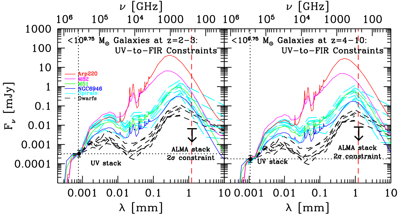
FIG. 9.— Illustration of the general constraints we can set on the overall shape of the near-UV + far-infrared spectral energy distribution for lower-mass ( < 10^{9.75} M_{\odot} ) galaxies at z = 2-3 (left panel) and z = 4-10 (right panel) based on the results we obtain by stacking our deep 1.2 mm ALMA HUDF observations at the positions of candidate z = 2-10 galaxies. The flux points at \sim 0.8 and 1.1 \mu\text{m} shows the UV flux for our lower-mass stack of z = 2-3 and z = 4-10 candidates, respectively, while the large upper limit shows the 2\sigma upper limit we can set on the flux at 1.2 mm (which is just a factor of 20 and 44 higher, respectively, than the weighted flux in the UV continuum that contributes to the stack results shown here: see Table 12 from Appendix D). For reference, we have included model SED templates from Silva et al. (1998), Dale et al. (2007), and some lower-metallicity galaxies studied in the KINGFISH project (Dale et al. 2012) redshifted to z \sim 4 . Our ALMA observations suggest that faint high-redshift galaxies show less dust emission at 1.2 mm than any of these SED templates.
