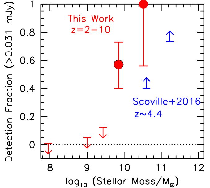
FIG. 5.— Fraction of tentatively detected ( >2\sigma ) z = 2-10 galaxies in our ALMA 1.2 mm continuum observations versus the inferred stellar mass (solid red circle). Errors and upper limits are 1\sigma . Only the 172 z = 2-10 galaxies where our 2\sigma continuum sensitivity is highest ( <34\mu\text{Jy} ) are included in this determination. The blue upward arrows are from Scoville et al. (2016) and indicate lower limits on the detected fraction (i.e., at >0.031 mJy) based on the results of that study. Stellar mass appears to be a very good predictor of dust emission in z = 2-10 galaxies, with 5 of the 8 > 10^{9.75} M_{\odot} galaxies probed at the requisite sensitivity being detected at >2\sigma (and several other > 10^{9.75} M_{\odot} galaxies probed by our field show measured 1.2 mm fluxes consistent with the other measurements).
