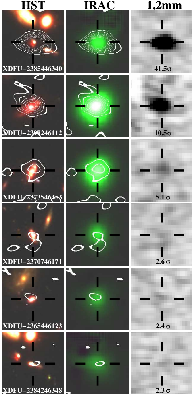
FIG. 4.— HST B_{435i775}H_{160} (left), IRAC 3.6\mu\text{m} (middle), and 1.2 mm ALMA-continuum images (right) for six z \sim 2-3 galaxies that we detect ( >3.5\sigma ) or tentatively detect ( >2\sigma ) in our 1 arcmin 2 deep ALMA map over the HUDF. The size of the stamps is 7.2'' \times 7.2'' . The position of our 1.2 mm-continuum detections relative to the position of sources in our HST or Spitzer /IRAC images are illustrated in the left and center stamps with the 2\sigma , 4\sigma , 6\sigma , 8\sigma , and 10\sigma contours (white lines). Light from neighboring sources on the IRAC images have been removed for clarity. Significantly enough, these sources are among the 13 z = 2-10 candidates from that 1 arcmin 2 region with the highest stellar mass estimates. All six have estimated stellar masses \geq 10^{9.75} M_{\odot} . Given evidence that dust emission from star-forming galaxies correlates with stellar mass in many studies (e.g., Pannella et al. 2009, 2015; Reddy et al. 2010; Whitaker et al. 2014; Álvarez-Márquez et al. 2016), these sources are amongst the 6 sources most likely to show dust emission from our entire z = 2-10 LBG selection. The fact that each of them shows ALMA flux at \geq 2.3\sigma seems to confirm that stellar mass is an especially useful predictor of dust emission for normal star-forming galaxies at z \gtrsim 2 . Each of these sources also shows evidence for being detected ( \gtrsim 2\sigma ) in the MIPS 24\mu\text{m} observations (Table 10 from Appendix B).
