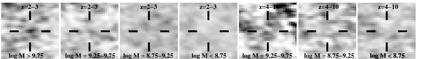
FIG. 7.— Stacked 1.2mm-continuum images ( 9'' \times 9'' ) for all candidate z = 2 - 3 and z = 4 - 10 galaxies falling in four different ranges of stellar mass ( < 10^{8.75} M_{\odot} , 10^{8.75} to 10^{9.25} M_{\odot} , 10^{9.25} to 10^{9.75} M_{\odot} , and > 10^{9.75} M_{\odot} ). In the stacks, sources are weighted according to the square of their UV flux and the inverse square of the noise. The 3 sources from this analysis individually detected at >4\sigma are not included in the stack results shown in this figure.
