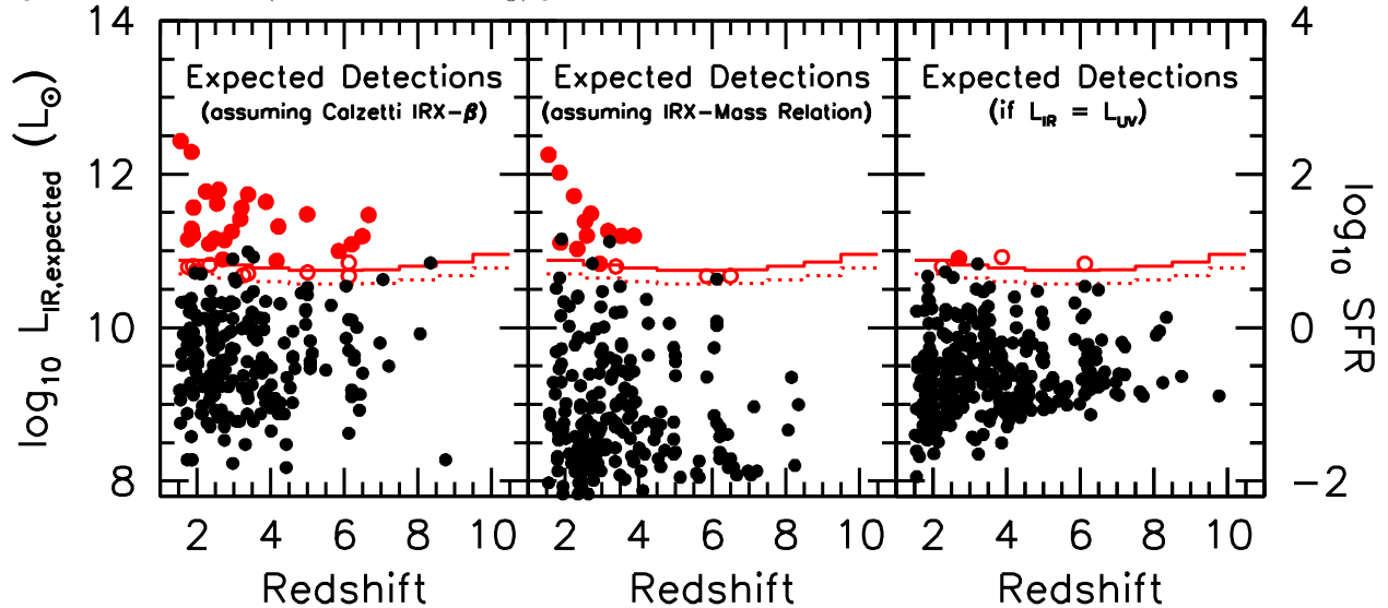
FIG. 3.— Expected IR luminosities (in L_{\odot} ) versus photometric redshift of z = 2-10 galaxies (solid circles) within the 1 \text{ arcmin}^2 ASPECS region. Expected IR luminosities are based on (1) the M99 IRX- \beta relationship (left panel), (2) the approximate z \sim 2-3 IRX-stellar mass relationship (center panel: see Appendix A), or (3) assuming L_{IR} = L_{UV} (right panel). The solid and dotted red lines indicate the 3\sigma and 2\sigma limiting luminosities, respectively, to which we can probe as a function of redshift in the deepest regions within our 1 \text{ arcmin}^2 field (assuming that the SED is well represented by a 35 K-modified blackbody). The solid and open red circles correspond to sources where 3\sigma and 2\sigma detections are expected, respectively, adopting the assumptions from a given panel, while the black circles indicate sources where a tentative 2\sigma detection is not expected. Black sources can appear above the red lines if these sources fall in regions of ASPECS where the sensitivities are lower than the maximum.
