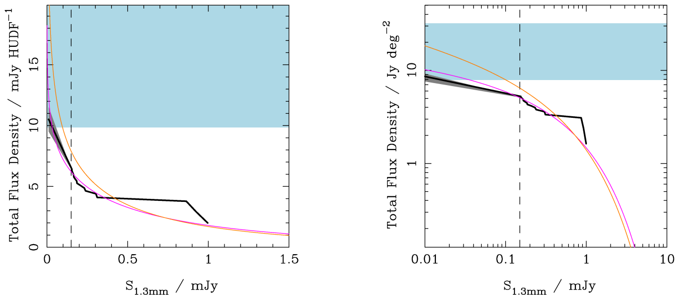
Figure 10. Total integrated flux density at \lambda = 1.3 mm. The left-hand plot shows results per HUDF (i.e. per 4.5 \text{ arcmin}^2 ) in linear units, while the right-hand plot shows the more standard logarithmic representation in units of \text{Jy deg}^{-2} . The solid black line in each plot shows simply the running sum of the flux densities of the 16 ALMA HUDF sources, starting at the total contributed by sources brighter than S_{1.3} = 1 \text{ mJy} (i.e. \simeq 0.8 \text{ Jy deg}^{-2} ; Scott et al. 2012) and summing down to our (effective) detection threshold of S_{1.3} = 0.15 \text{ mJy} (marked by the vertical dashed line in both plots). Below that flux density, we extrapolate the black line (with grey shading to indicate the uncertainty) to account for the contribution estimated from our stacking analysis, which samples the fainter population down to S_{1.3} \simeq 0.01 \text{ mJy} (and adds an additional 4.1 \pm 1.0 \text{ mJy / HUDF} ). The blue-grey shaded region in both panels indicates the (highly-uncertain) estimate of the 1.3-mm background as measured by COBE (i.e. 17^{+16}_9 \text{ Jy deg}^{-2} ; Puget et al. 1996; Fixsen et al. 1998). It can be seen that our HUDF derived flux-density total is (just) consistent with the 1\text{-}\sigma lower bound on the background estimate. The magenta and orange curves give the predicted background as a function of 1.3-mm flux-density for the scaled Schechter number-count models of Hatsukade et al. (2016) and Fujimoto et al. (2016) already utilised in Fig. 3, and discussed in Section 5.2. Our results can be plausibly reconciled with those of Hatsukade et al. (2016), but to achieve the much higher estimated backgrounds reported by Fujimoto et al. (2016) or Carniani et al. (2015) down to S_{1.3} = 0.01 \text{ Jy} we would require an approximate doubling of the flux density we have actually been able to uncover in the HUDF through source detection and stacking.
