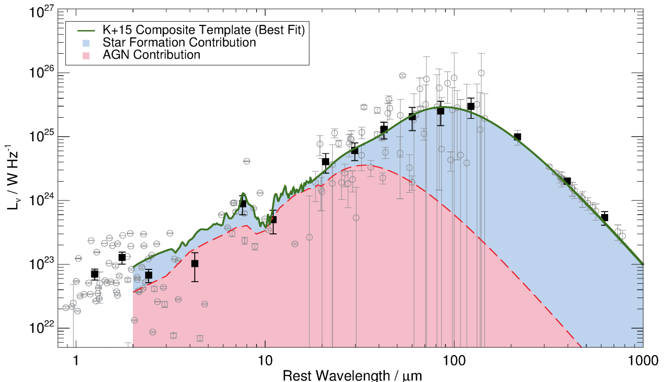
Figure 7. The combined Spitzer + Herschel +ALMA photometry of the 16 ALMA sources, (after de-redshifting and scaling to the same rest-frame 1.3-mm luminosity), fitted by the composite star-forming+AGN template of Kirkpatrick et al. (2015). The solid black squares indicate the weighted mean of the scaled multi-source photometry within a given wavelength bin. The accuracy of the redshift information results in the 8- \mu m feature being clearly visible in the observed combined rest-frame SED. The best-fitting composite template has an AGN component which contributes only \simeq 20\% to the bolometric rest-frame far-infrared (8 – 1000 \mu m) luminosity, and is completely negligible at the wavelengths sampled by the ALMA imaging.
