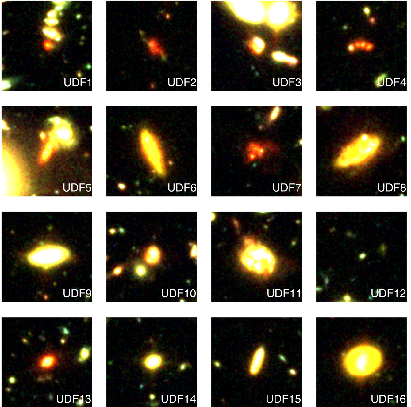
Figure 4. Colour ( i_{775}+Y_{105}+H_{160} ) HST postage-stamp images of the 16 ALMA-detected galaxies listed in Table 1. Each stamp is 6 \times 6 arcsec in size, with North to the top, and East to the left.
