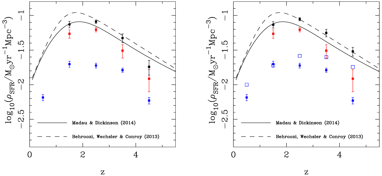
Figure 13. The cosmic evolution of comoving star-formation rate density, \rho_{SFR} . In the left-hand panel we plot our new ALMA-derived estimates of \rho_{SFR} (obscured) (red points), estimated values of \rho_{SFR} (visible) produced by summing the raw UV-derived star-formation rates of the galaxies in the HUDF (blue points), and the values of \rho_{SFR} (total) that result from adding these two contributions at each redshift (black points). The solid and dashed curves show two recent parametric descriptions of the evolution of \rho_{SFR} as derived from the literature by Madau & Dickinson (2014) and Behroozi, Wechsler & Conroy (2013) respectively (scaled to the IMF of Chabrier 2003). In the right-hand panel we show the impact of including a more complete census of \rho_{SFR} (visible), based on the luminosity-weighted integral of the evolving UV galaxy luminosity function, down to M_{UV} = -15 (Parsa et al. 2016; Bouwens et al. 2015). In this panel the values of \rho_{SFR} (obscured) are unchanged, but the black points indicating \rho_{SFR} (total) now include the more complete (and, at high redshift, higher) census of \rho_{SFR} (visible), as shown by the open blue squares. At z \simeq 2 the agreement with the parametric fit provided by Behroozi et al. (2013) is excellent, and our results indicate that there is a transition from \rho_{SFR} (visible) / \rho_{SFR} (obscured) > 1 , to \rho_{SFR} (visible) / \rho_{SFR} (obscured) < 1 at z \simeq 4 .
