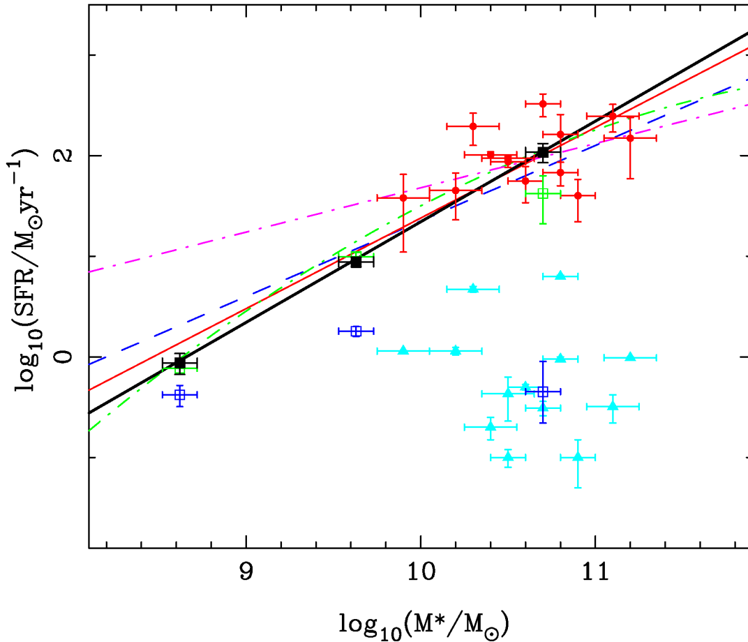
Figure 11. Star-formation rate versus galaxy stellar mass at z \simeq 2 . The 13 ALMA sources that lie in the redshift range 1 < z < 3 (median redshift z = 2.09 ) are shown twice, first adopting the total star-formation rate (i.e. UV+FIR SFR; red points) and then adopting only the raw UV SFR (cyan triangles). Also shown is the average value in 3 stellar-mass bins at 1 < z \leq 3 (derived from stacking as described in the text) for total UV+FIR SFR (black solid squares), raw UV SFR (navy-blue open squares), and dust-corrected SFR (from the optical–near-infrared SED fitting; green open squares). The binned points are plotted at the median stellar mass of each bin. Reassuringly, the green and black values agree well in the two lower-mass bins, but the SED A_V -corrected values fall about a factor of 2 short of the true ALMA-derived average in the highest mass bin. The solid black line shows a simple relation of the form \text{SFR} \propto M_*^{1.0} , with \text{sSFR} = 2.2 \text{ Gyr}^{-1} . The other curves are proposed fits to the ‘main-sequence’ of star-forming galaxies, at z \simeq 2 , published by Daddi et al. (2007; solid red line, after conversion to a Chabrier IMF), Whitaker et al. (2012; dot-dashed magenta line), Whitaker et al. (2014; dot-dashed green curve), and Speagle et al. (2014; dashed blue line).
