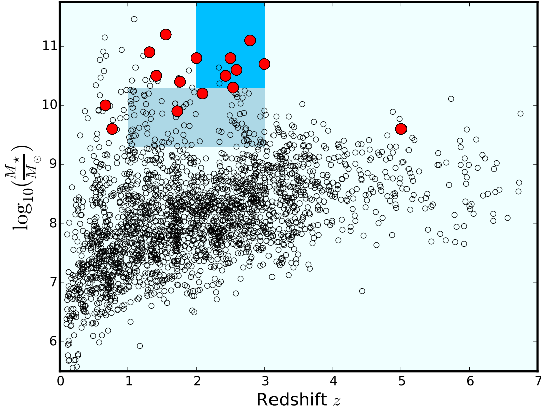
Figure 6. Stellar mass versus redshift for the galaxies in the HUDF, highlighting (in red) those detected in our ALMA 1.3-mm image. The connection between dust-enshrouded SFR and M_* is clear, and indeed, as emphasized by the bright-blue box at the top of the plot, we detect 7 of the 9 galaxies (i.e. \simeq 80\% ) with M_* \geq 2 \times 10^{10} M_\odot at z > 2 . Also apparent is the emergence of a significant population of quenched high-mass galaxies at 1 < z < 2 , where the ALMA detection rate for galaxies with M_* \geq 2 \times 10^{10} M_\odot drops to 5/19 (i.e. \simeq 25\% ). It can be also seen that the lack of ALMA detections beyond z > 3 in our sample simply reflects the dearth of comparably-massive galaxies in the HUDF at these redshifts (due to the evolution of the galaxy stellar mass function). The blue-grey rectangle indicates the sample of \simeq 90 galaxies in the redshift range 1 < z < 3 and mass range 9.3 < \log_{10}(M_*/M_\odot) < 10.3 used to produce the stacked ALMA image shown in Fig. 8, and discussed in Section 7.
