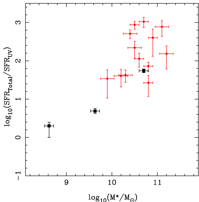
Figure 12. The ratio of total SFR (i.e. UV+FIR) to UV-visible SFR as a function of galaxy stellar mass at z \simeq 2 . The individual ratios for the 13 ALMA-detected sources at 1 < z \leq 3.0 are indicated by the red points, and the median value at \log_{10}(M_*/M_\odot) > 10.3 is \simeq 200 (see column 9 in Table 4). The black squares indicate the ratios for each of our three mass bins, summing all SFR (detected-FIR + stacked-FIR + total-UV) in each bin, and dividing by all the raw UV SFR in that mass bin. The stacked (true total ratio) value at median mass \log_{10}(M_*/M_\odot) = 10.7 is 55 \pm 6 (significantly lower than the median ratio of ALMA-detected sources). The average ratio at \log_{10}(M_*/M_\odot) = 9.6 is 4.9 \pm 0.8 , while at \log_{10}(M_*/M_\odot) = 8.6 our analysis yields 2.5 \pm 1 (see Section 8.2).
