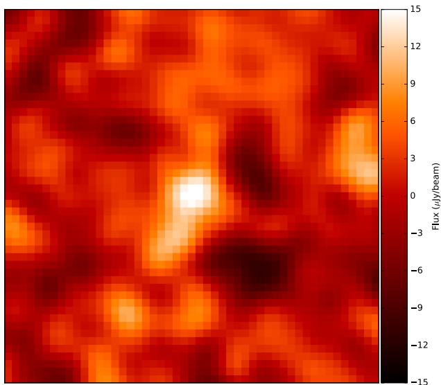
Figure 8. The result of stacking the ALMA imaging on the positions of galaxies in the redshift range 1 < z < 3 and the stellar mass range 9.3 < \log_{10}(M_*/M_\odot) < 10.3 , (excluding the sources already detected and listed in Table 4). The image shown is 5.9 \times 5.9 arcsec. The stacked ‘source’ includes 89 galaxies, and has a mean flux density (point-source + 25%) of S_{1.3} = 20.1 \pm 4.6 \mu\text{Jy} , corresponding to a mean SFR of 6.0 \pm 1.4 M_\odot \text{yr}^{-1} . This means that galaxies in this mass and redshift range contribute a total dust-enshrouded SFR \simeq 530 \pm 130 M_\odot \text{yr}^{-1} . The same sources have an average UV luminosity corresponding to an absolute magnitude of M_{UV} = -19.38 , and hence contribute a total unobscured (raw UV) SFR \simeq 160 M_\odot \text{yr}^{-1} . These results imply an average ratio of obscured:unobscured SFR of \simeq 3.3 (or total-SFR/unobscured-SFR \simeq 4.3 ), and a sSFR \simeq 1.95 \text{Gyr}^{-1} at a median mass of \log_{10}(M_*/M_\odot) = 9.6 and median redshift z = 1.92 .
