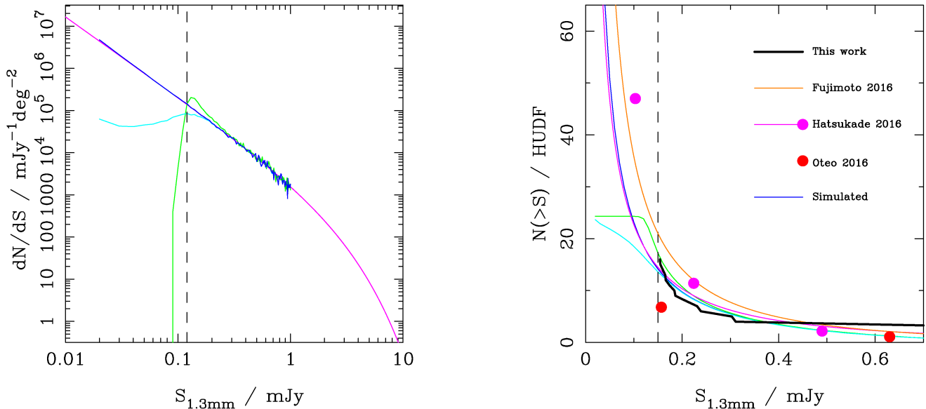
Figure 3. Left: Completeness and flux boosting in the HUDF ALMA 1.3-mm image. The magenta curve shows the differential number counts as given by the Schechter-function fit of Hatsukade et al. (2016), shifted from 1.1-mm to 1.3-mm by scaling flux density down by a factor of 1.65 (Fujimoto et al. 2016). The navy blue line shows the results of randomly drawing 1000 HUDF-size samples from this number-count model, and so represents the input for our source-injection simulations. The green curve shows the number counts as retrieved from the 1000 ALMA HUDF images using the same source extraction technique as applied to uncover the real sources, and insisting on S/N > 3.5 . The cyan curve shows the same retrieved sources, but at their input rather than retrieved flux densities. The vertical dashed line indicates our chosen point-source detection threshold of S_{1.3} = 0.120 mJy, where it can be seen that flux boosting almost perfectly offsets the effect of incompleteness. Right: Cumulative number counts scaled to the size of the HUDF. The results from the present study are plotted as the thick black line (after scaling by a factor of 1.25 to account for average resolved flux density), and compared with the results of other recent studies (scaled to 1.3-mm) as indicated in the legend. We found \simeq 1.5 times sources than anticipated given the number counts from Fujimoto et al. (2016) (orange curve), and also found fewer sources than indicated by the binned cumulative number counts reported by Hatsukade et al. (2016) (magenta points). However, our ALMA HUDF counts are in good agreement with integration of the Schechter fit to the differential counts provided by Hatsukade et al. (2016) (magenta line), and lie above the recent number-count results reported by Oteo et al. (2016) (red points), which were based on higher significance cuts, and arguably less biased pointings than the afore-mentioned studies. As in the left-hand panel, our simulated number counts are indicated by the navy blue line, and the impact of flux boosting+incompleteness is indicated by the green curve, with incompleteness indicated in cyan. Extrapolation of this model to still fainter flux densities suggests that to uncover \simeq 100 1.3-mm sources in the HUDF would require reaching a detection limit of S_{1.3} = 30 \mu\text{Jy} (i.e. \simeq 4 times deeper than achieved here).
