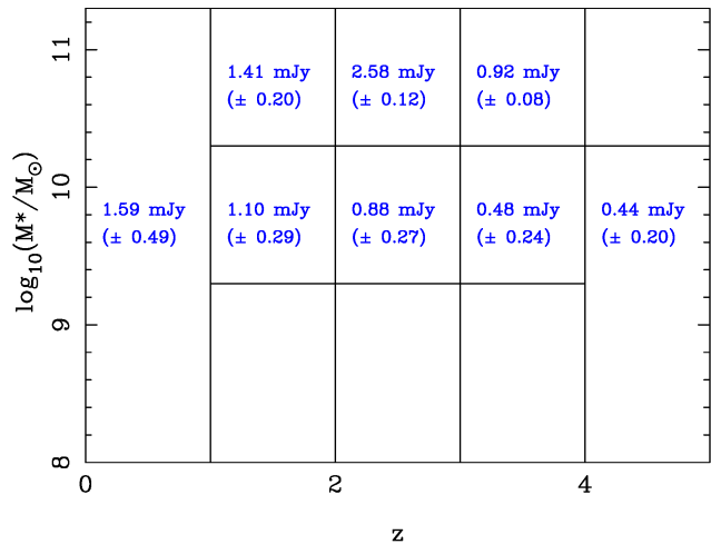
Figure 9. The distribution of 1.3-mm flux density found within the HUDF across the galaxy redshift–star-mass plane. The figures given here combine the flux densities of the detected sources and the results of stacking in the appropriate redshift-mass bins (excluding detected sources to avoid double counting). Results are only given for bins within which stacking yielded better than a 2\text{-}\sigma detection, typically corresponding to an average flux-density S_{1.3} \geq 0.010 \text{mJy} . At z > 4 the HUDF contains no galaxies more massive than \log_{10}(M_*/M_\odot) = 10.3 , and so the right-hand cell in the top row is genuinely blank. The cells below \log_{10}(M_*/M_\odot) = 9.3 at 1 < z < 3 may contain additional 1.3-mm flux density, but not at a level that could be securely detected via stacking in the current image. At z < 1 and z > 4 , low sample size precludes bin subdivision by mass, and so we simply give the total flux detected via stacking of all sources in the z < 1 and z > 4 redshift bins. Addition of all the numbers in this figure, combined with an estimated contribution of \simeq 1 \text{mJy} per HUDF from sources brighter than S_{1.3} \simeq 1 \text{mJy} (equivalent to 0.8 \text{Jy deg}^{-2} ) gives an estimate of 10.6 \pm 1.0 \text{mJy} for the 1.3-mm flux density in the HUDF down to S_{1.3} \simeq 0.01 \text{mJy} (equivalent to 8.5 \pm 0.9 \text{Jy deg}^{-2} ; see Fig. 10). Of this total estimated background, \simeq 70\% is provided by sources with \log_{10}(M_*/M_\odot) > 9.3 in the redshift range 1 < z < 3 . Within our background estimate, \simeq 45\% of the flux density is contributed by the 16 individually-detected sources in our ALMA image of the HUDF, with only \simeq 35\% added by our attempts to extend flux retrieval down to \simeq 0.01 \text{mJy} sources through stacking.
