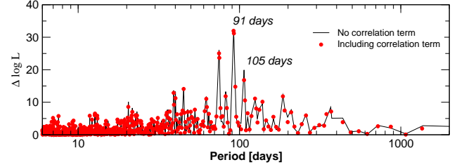
Fig. 6. Log-likelihood periodograms for planet d (91 days) including the correlation term (red dots) compared to the original periodogram without them (black line). The inclusion of the correlation term increases the contrast between the peaks at 91 and 105 days, favoring the interpretation of the 91 days signals as a genuine planet candidate.
