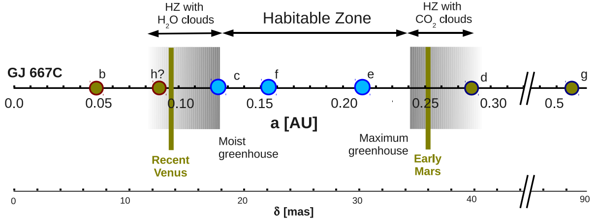
Fig. 15. Liquid water habitable zone of GJ 667C with the proposed seven candidates as estimated using updated relations in Kopparapu et al. (2013). Three of the reported planets lie within the HZ. The newly reported planets f and e are the most comfortably located within it. The inner edge is set by the moist greenhouse runaway limit and the outer edge is set by the snow ball runaway limit. The empirical limits set by a recent uninhabitable Venus and an early habitable Mars are marked in brown solid lines. The presence of clouds of water (inner edge) or CO 2 (outer edge) might allow habitable conditions on planets slightly outside the nominal definition of the habitable zone (Selsis et al. 2007).
