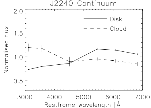
Fig. 6.— By integrating the faint continuum over large wavelength ranges, excluding emission lines, we probe the photometric properties of the continuum. The Cloud is bluer than the Disk.
