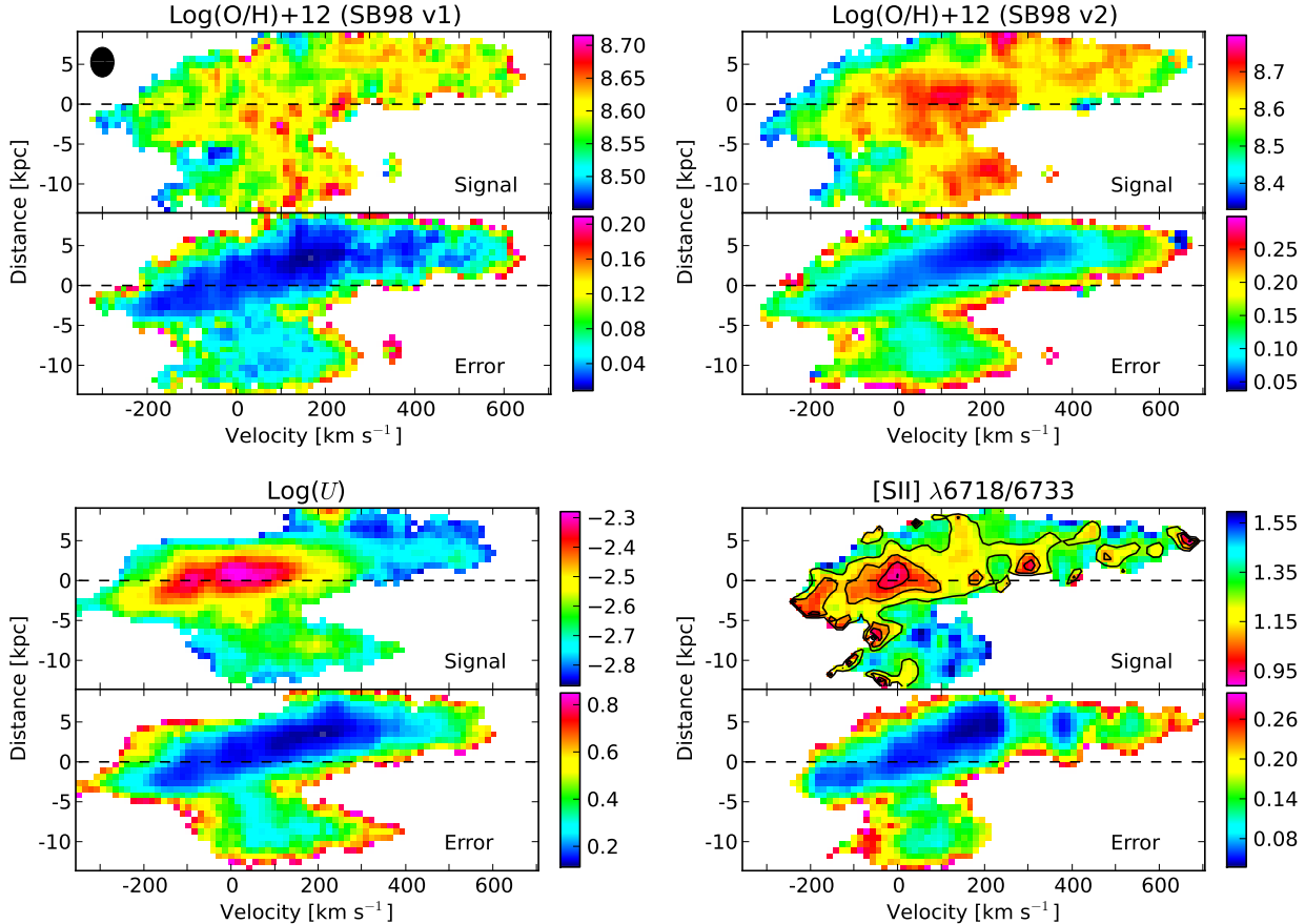
Fig. 5.— Top row: Oxygen abundance, estimated using the two strong line diagnostics of Storchi-Bergmann et al. (1998). Bottom left: Ionization parameter. Bottom right: [SII] line ratio (map) and electron density (contours) for T_e = 13000 K. Contour levels are drawn at n_e = 150, 300, 450, 600 \text{ cm}^{-3} .
