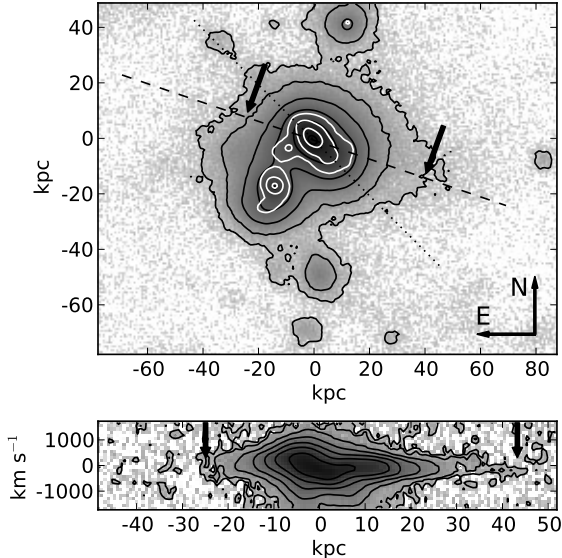
Fig. 8.— Deep GMOS r -band image (top) of J2240 revealing the extended halo. The dashed line indicates the position angle of the spectrum (bottom, showing the [OIII] line), the two arrows out to which radius we detect [OIII]. Black contour lines are logarithmically spaced. Contours (white) of the CFHT image (Fig. 1) and the XSHOOTER slit (dotted line) are overplotted for reference.
