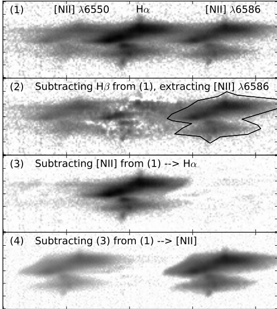
Fig. 2.— Deblending the H\alpha -[NII] line complex (panel 1). Panel 2: A rescaled and smoothed version of H\beta is subtracted, and [NII] \lambda 6586 extracted within a closed polygon line. Panel 3: [NII] gets smoothed and subtracted from the original line complex, leaving H\alpha isolated. Panel 4: H\alpha gets smoothed and subtracted from the original line complex, leaving the [NII] doublet.
