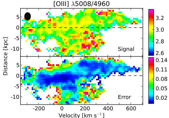
Fig. 3.— The [OIII] j_{\lambda 5008}/j_{\lambda 4960} ratio (theoretical value: 2.98) is constant within errors. The black ellipse shows the spatial and spectral scale beyond which data points become statistically independent (same for all other similar plots). The dashed line indicates the spatial location of highest continuum flux (coincident with the nucleus). The origin of the velocity axis coincides with the location of highest electron density (see Sect. 4.2).
