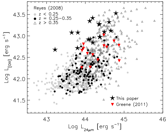
Fig. 9.— [\text{OIII}]\lambda 5008 vs. WISE 24\mu\text{m} luminosities. GBs are shown by asterisks, and the red triangles represent the luminous obscured quasars studied by Greene et al. (2011). The other data points show the type-2 AGN sample from Reyes et al. (2008) for three different redshift bins, with black dots covering the same redshift range as GBs. At a given L_{24\mu\text{m}} , GBs have 5 – 50 times higher L_{[\text{OIII}]} than other type-2 AGN.
