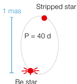
Binary scenario
