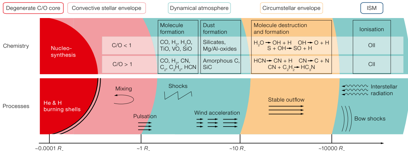
Figure 3. Schematic diagram of an asymptotic giant branch star from interior to circumstellar environment, showing the chemical and physical processes involved in mass loss. VLT instrumentation (PIONIER, GRAVITY and MATISSE) can resolve these stars from their surfaces (at 1 R_{\odot} ) to their circumstellar envelopes (out to \sim 10 R_{\odot} ), probing convection, pulsation, shocks and dust formation. ALMA can resolve the circumstellar environment and molecular processes. VLT imaging at high angular resolution accesses the outer scales ( 100\text{--}1000 R_{\odot} ). Reproduced here with permission of S. Lijjengre.
