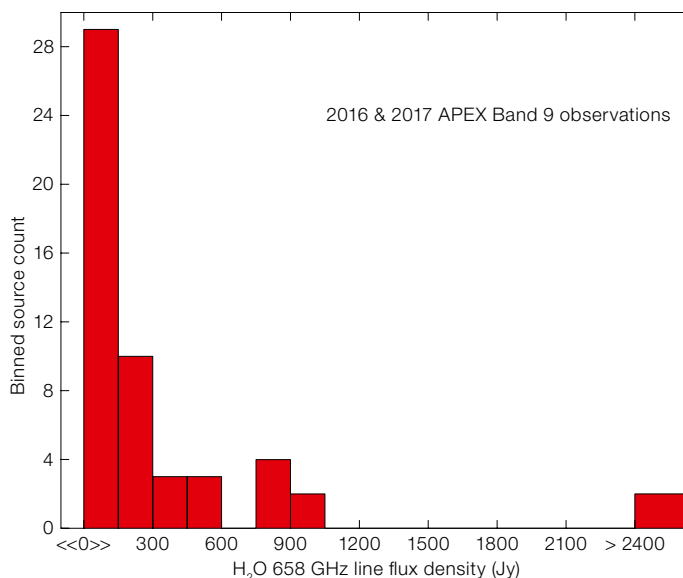
Figure 3. Histogram showing the 658 GHz line flux density of ortho-water for all sources observed with APEX in 2016 and 2017. The first bin from \ll 0 \gg –150 Jy starts at the 3\text{-}\sigma level, at \sim 29 \text{ Jy} .
