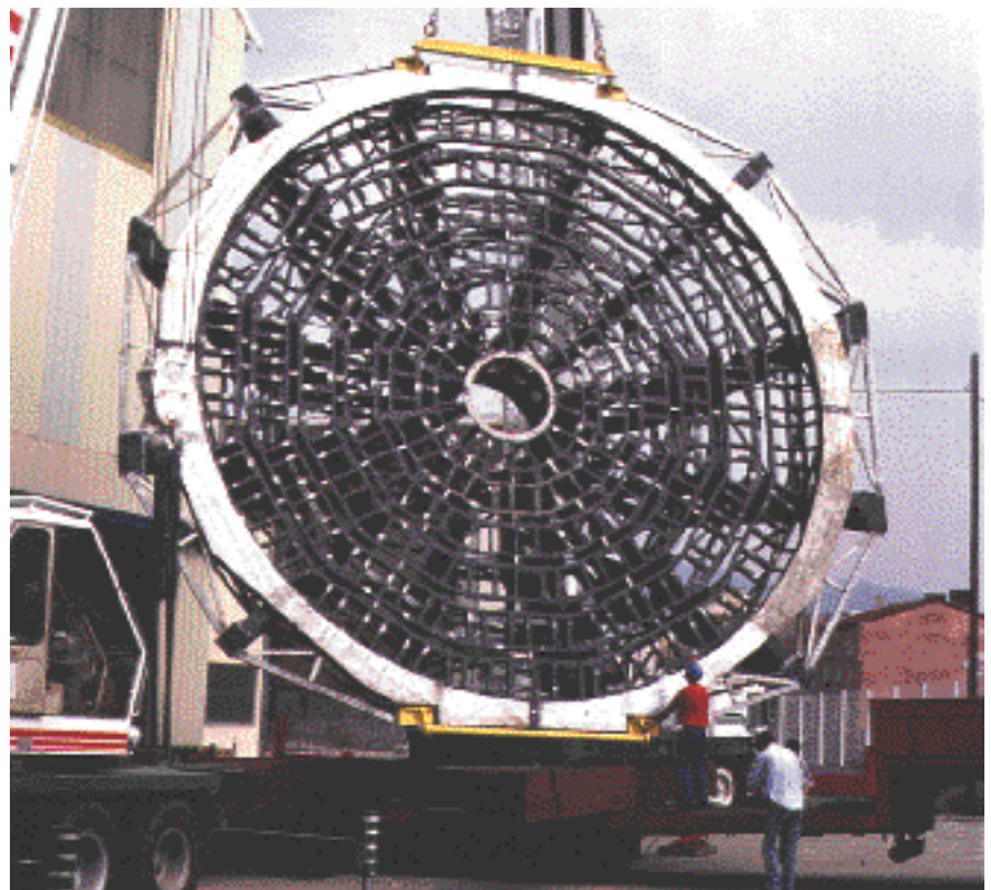
► The primary mirror cell of the VLT (Unit 1) is turned at the St-Chamond GIAT factory, prior to undergoing dimensional check and painting (16/07/96).
