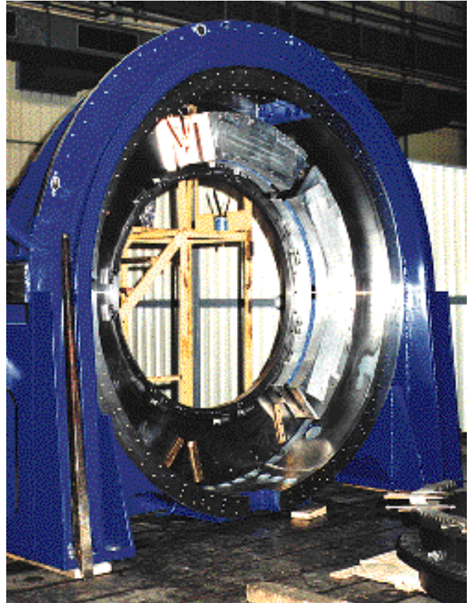
Figure 4: Altitude drive pre-assembling. ▶
