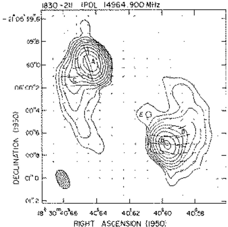
Figure 1: VLA image of PKS1830-211 at 15 GHz (from Subrahmanyam et al. 1990), showing contours of the flux and the electric field polarisation vectors.
