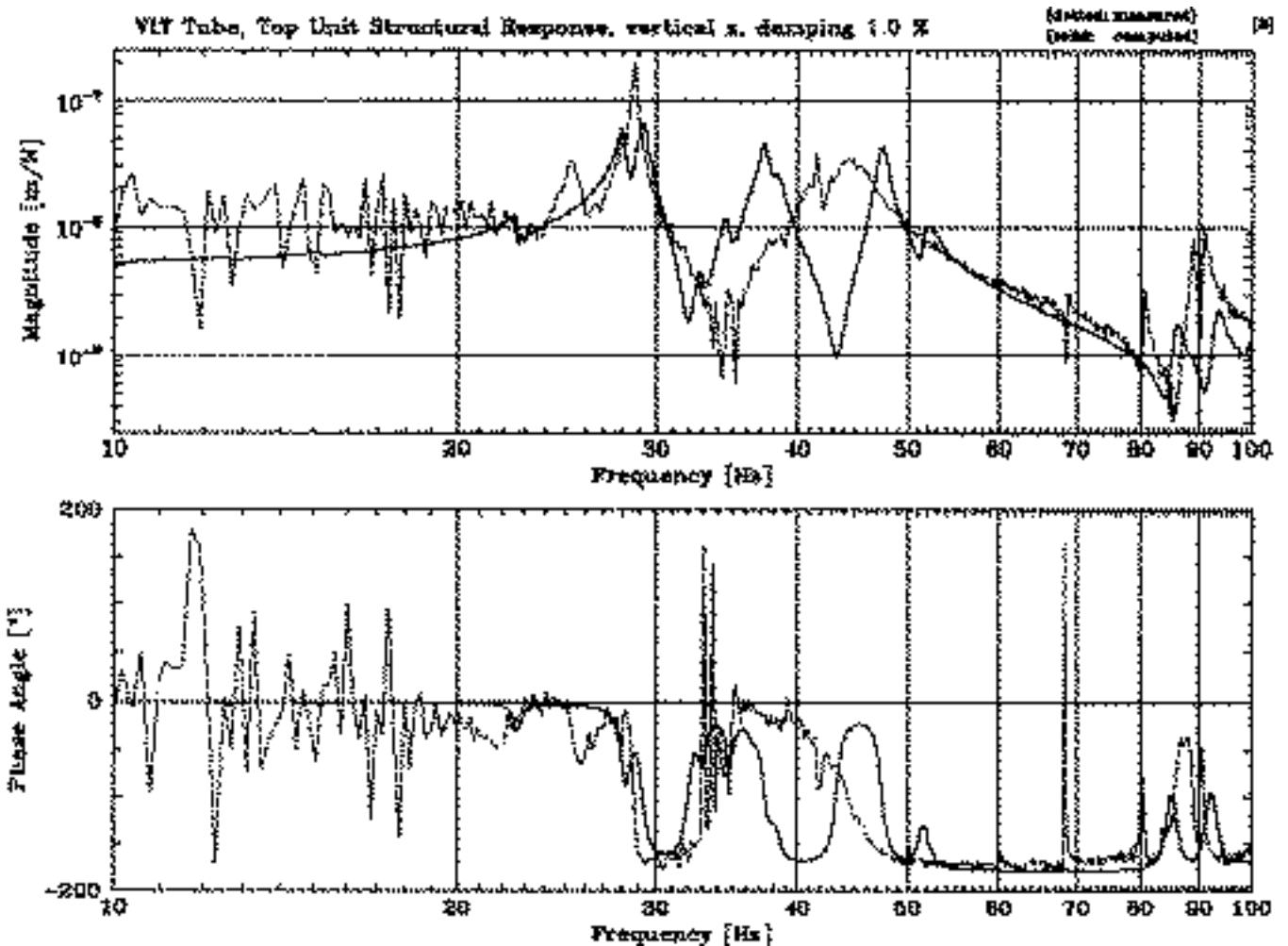
Figure 5: Top unit dynamic performances 1% damping (Koehler, Koch, Quattri).
