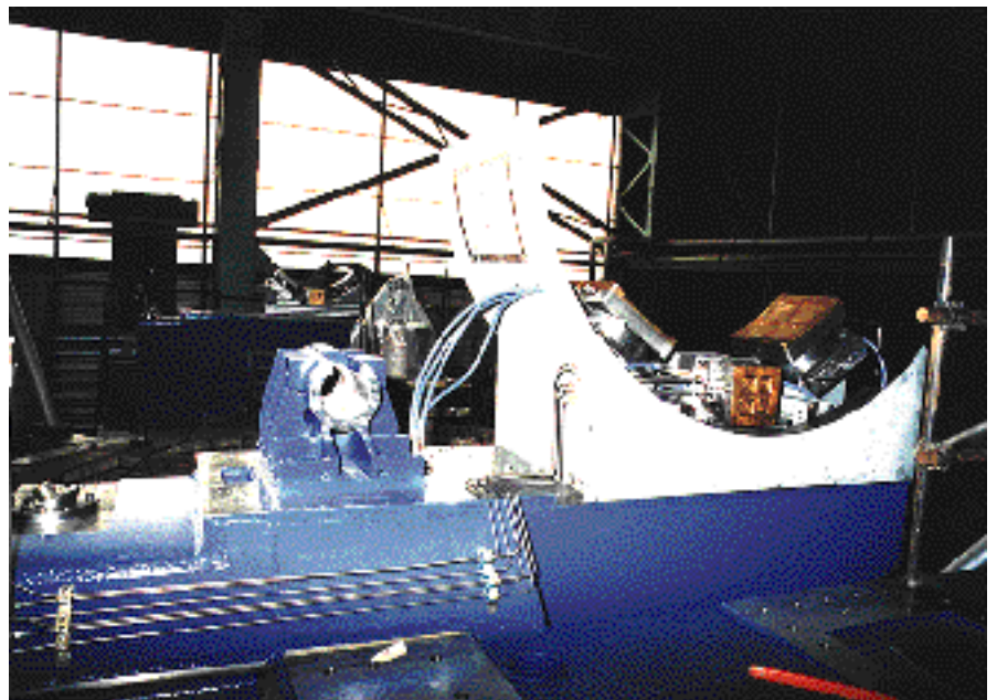
Figure 3: Altitude hydrostatic bearing pads and locking pin support.
