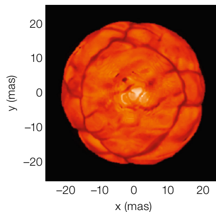
Figure 2. Intensity map of the best-matching snapshot of a radiative hydrodynamics simulation of Betelgeuse at 2.2 \mu\text{m} based on AMBER observations. From Montargès et al. (2014).
