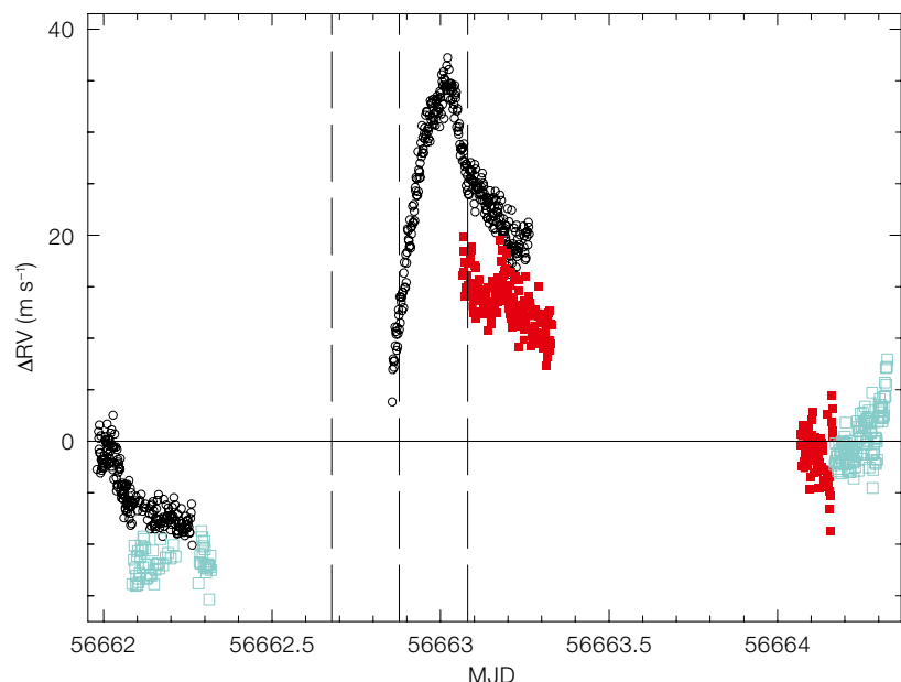
Figure 3. Radial velocities measured with HARPS on 4–6 January 2014. Open black circles are observations of Europa from La Palma while colour squares are the observations of Ganymede (cyan) and Europa (red) from La Silla. A constant offset of 107.5 m s -1 , as measured far from the transit, is taken as the instrumental baseline and was subtracted from the data. The vertical dashed lines mark the expected ingress and egress of the Earth's transit as seen from Europa.
