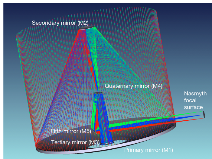
Figure 7. Optical layout for the Nasmyth configuration of the E-ELT.
