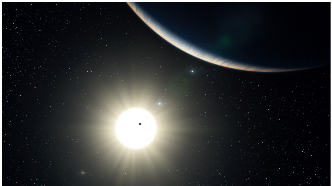
Figure 2. An artist's conception of a multi-planet system as they are commonly found now around nearby stars.
