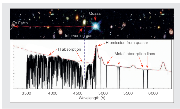
Figure 5. The light of distant quasars is absorbed by a variety of components of the Universe on its way to Earth.
