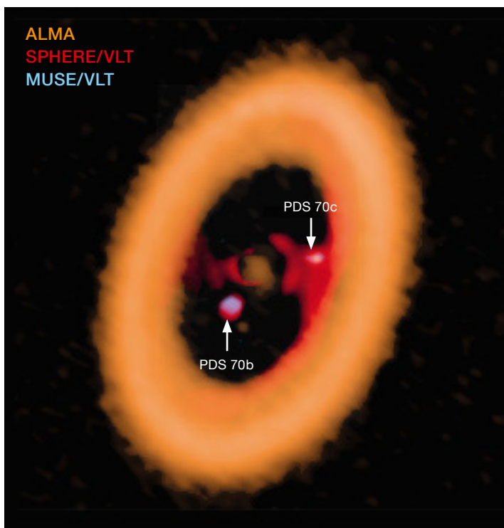
An image of the young stellar system obtained from ALMA 855- \mu\text{m} continuum observations (yellow), superposed on MUSE and SPHERE observations from the VLT in blue and red. The image clearly shows the circumstellar disc, and the two planets PDS 70b and PDS 70c. The circumplanetary disc is clearly visible in \text{H}\alpha emission from MUSE, indicating ongoing accretion; the ALMA continuum emission traces the circumplanetary dust. The spatial scale of the image is approximately 1.5 \times 2 arcseconds.
