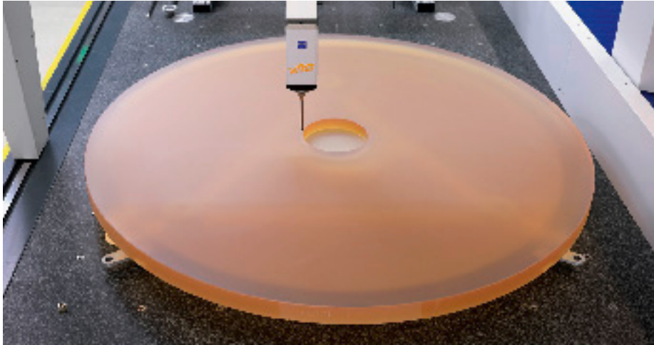
Top: One of the segment blanks for the primary mirror (M1), manufactured by SCHOTT for the ELT. Centre: The massive three-tonne blank for the ELT's secondary mirror (M2). Bottom: Engineers inspecting the blank for the ELT's tertiary mirror (M3) at Safran Reosc.
