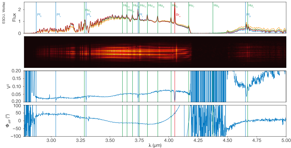
First GRA4MAT measurement for the Be star \delta Cen. The MATISSE fringes are stabilised by the GRAVITY fringe tracker, allowing long integration times in the L band, which is necessary to read the full L - M -band detector. Without GRA4MAT, MATISSE would be limited to only one 16-nm spectral window at a time.
