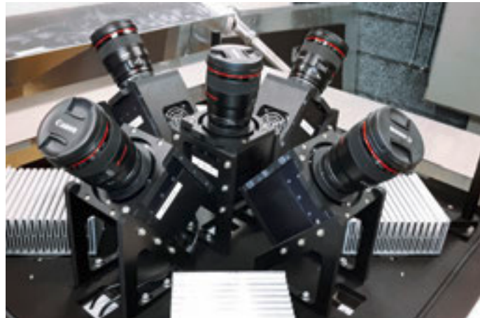
The MASCARA planet-hunting system at La Silla.
