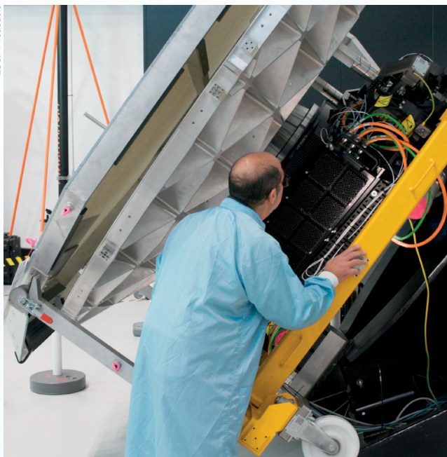
The M5 mirror support cell operating in the Large Integration Hall at ESO Headquarters.
