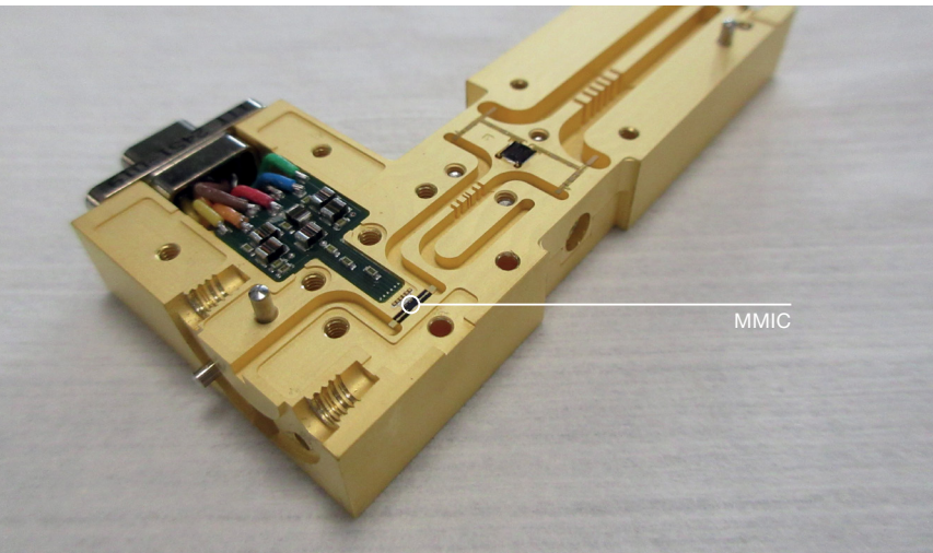
TASER Band 2 integrated low-noise amplifier and mixer. The monolithic microwave integrated circuit (MMIC) is labelled.
